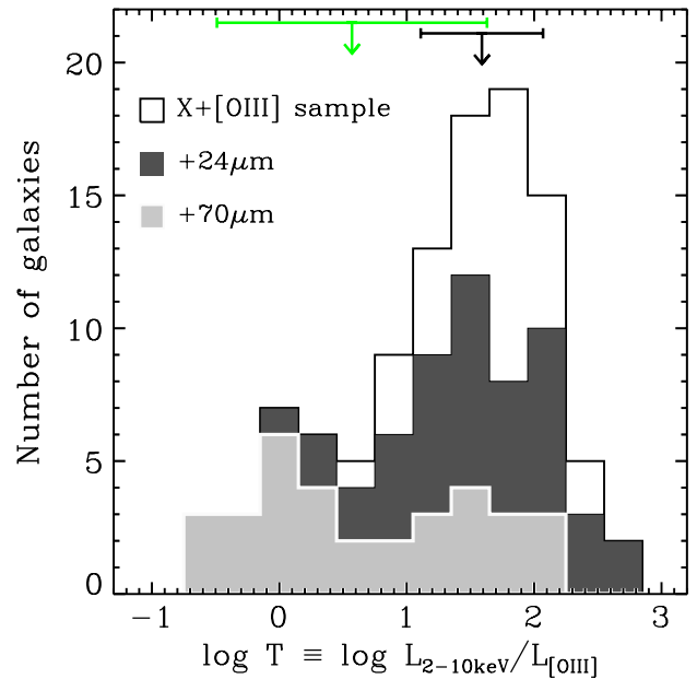
Figure 14. Distribution of the Compton-thickness parameter T \equiv L_{2-10\text{keV}}/L_{[\text{O III}]} for an X-ray+[O III]-selected sample of AGNs (black line). The distributions for the subsamples of galaxies detected at 24 \mu\text{m} and at 70 \mu\text{m} are overplotted in dark and light gray, respectively. The most absorbed systems (with lower values of T ) are preferentially detected at 70 \mu\text{m} . This subsample displays a much broader distribution of thickness parameter and a larger relative number of absorbed AGNs compared to both the 24 \mu\text{m} sample and the parent X-ray+[O III]-selected sample. The arrows at the top of the figure indicate the mean and standard deviation for nearby AGNs that are either obscured, Type 2 ( 0.59 \pm 1.06 dex; in green) or unobscured, Type 1 ( 1.59 \pm 0.48 dex; in black; Heckman et al. 2005).
