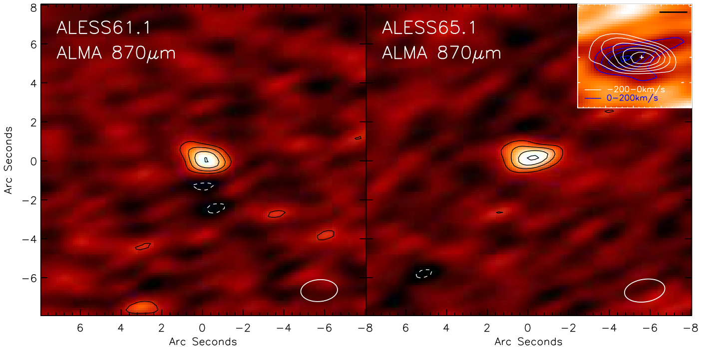
Figure 1. Top: 870 \mu\text{m} (345 GHz) velocity integrated ALMA maps of LESS61 and LESS65 from the Band 7 ALMA observations in compact configuration (these maps include the continuum and emission lines and are naturally weighted). In both cases, we detect strong 870 \mu\text{m} emission in both sub-millimeter sources associated with a single SMG. The r.m.s. noise in these maps is 0.44 and 0.42 mJy beam ^{-1} for LESS61 and LESS65 respectively. Contours denote \pm 3, 5, 7\dots\sigma . In each panel we also show the 50% contour of the synthesised beam which is approximately 1.8'' \times 1.2'' in both cases. These maps are centered at \alpha : 03\ 32\ 45.87 \delta : -28\ 00\ 23.3 and \alpha : 03\ 32\ 52.26 \delta : -27\ 35\ 26.3 for LESS61 and LESS65 respectively (Table 1). The inset in LESS65 shows the velocity structure in the [CII] in this source. The colour scale shows the (continuum subtracted) velocity integrated cube between -210 – 0 km s ^{-1} with the blue contours at 2, 3, 4, 5... \sigma . The white contours denote the velocity integrated emission 0 – 210 km s ^{-1} (also at 2, 3, 4, 5... \sigma ). The spatial offset between the blue-shifted and red-shifted emission in these two images is 0.50 \pm 0.25'' ( 3.3 \pm 1.7 kpc). If this spatial and velocity offsets represents rotating gas reservoir, then we estimate a dynamical mass of M_{\text{dyn}} \sim 3.5 \times 10^{10} \sin^2(i) M_{\odot} . In this inset, the solid bar shows a scale of 1'' .
