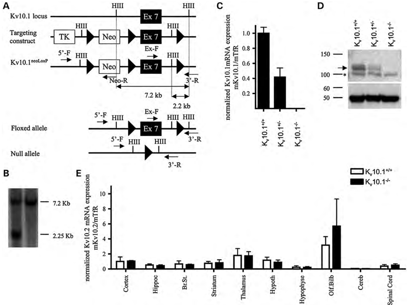
Figure 1. Generation and expression analysis of K_v10.1 -deficient mice. (A) Schematic representation of the K_v10.1^{+/+} locus, the targeting construct and the mutated alleles. K_v10.1^{neoLoxP} were bred with EllaCre transgenic mice to produce in vivo floxed allele and/or null allele due to an early expression of Cre recombinase during mouse embryo development. The probe for Southern blot analysis and primers for genotyping are indicated. (B) Southern blot analysis of K_v10.1 -ES cells ( HindIII digested) is shown. Bands corresponding to the different alleles are indicated (wild-type allele: 7.2 Kb K_v10.1 ; recombinant allele: 2.25 Kb K_v10.1 ). (C) Real time RT-PCR on cDNA was obtained from total brain RNA in K_v10.1^{+/+} , K_v10.1^{+/-} and K_v10.1^{-/-} mouse. The results indicate a complete deletion of K_v10.1 on K_v10.1^{-/-} animals. (D) Western blot using a polyclonal anti- K_v10.1 antibody did not detect specific signals in brain K_v10.1^{-/-} mice. The filled arrowhead marks the expected position for K_v10.1 ; non-specific bands are marked by an asterisk. Open arrowhead shows \alpha -tubulin used as a control. (E) Real time RT-PCR on cDNA obtained from cortex, hippocampus, brain stem, striatum, thalamus, hypothalamus, hypophysis, olfactory bulb, cerebellum and spinal cord from K_v10.1^{+/+} and K_v10.1^{-/-} mice. K_v10.2 expression is not regulated due to the absence of K_v10.1 in K_v10.1^{-/-} mice.
