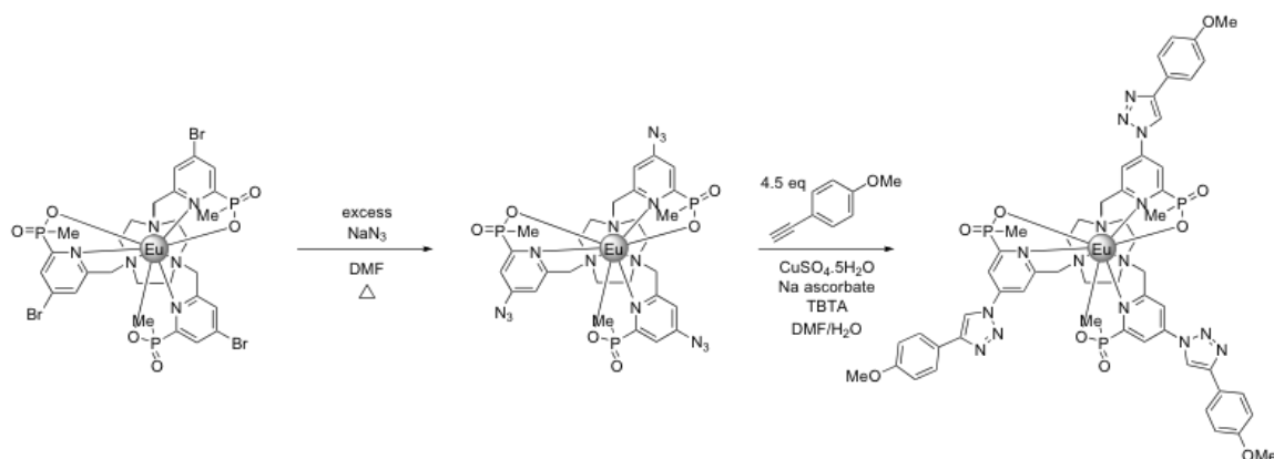
Scheme 1 Synthesis of the trispyridyl-triazole-anisole Eu(III) complex, [\text{Eu.L}^2]
