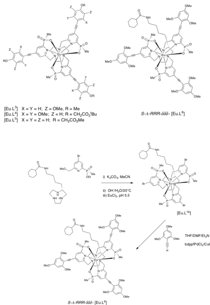
Scheme 2 Synthesis of the enantiopure complex [\text{Eu.L}^6]
