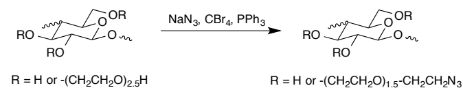
Scheme 1. Synthesis of partially ^{15}\text{N} -labelled \text{N}_3\text{-HEC}
