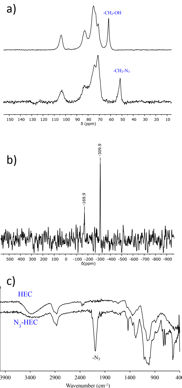
Fig. 2. Characterisation of \text{N}_3\text{-HEC} : a) solid state ^{13}\text{C} CP-MAS NMR spectra of HEC ( top ) and \text{N}_3\text{-HEC} ; b) solid state ^{15}\text{N} CP-MAS NMR spectrum of \text{N}_3\text{-HEC} ; c) FTIR spectra of HEC ( top ) and \text{N}_3\text{-HEC} .
