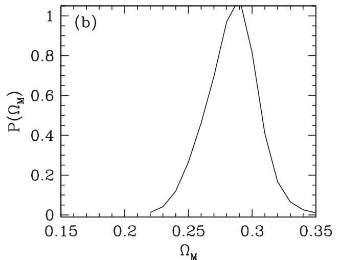
Figure 6. Marginalized posterior probability distribution of \sigma_8 in panel (a) and of \Omega_M in panel (b) from fitting the two-point galaxy correlation function.
