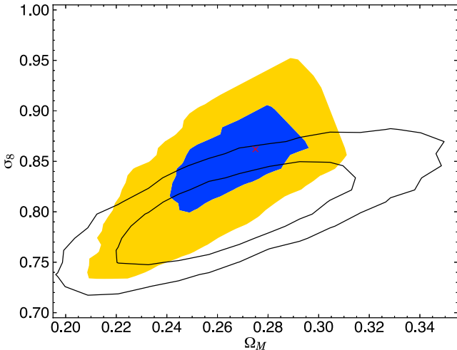
Figure 12. Joint constraint in the \sigma_8 – \Omega_M plane. The inner contour shows the boundary of the 68 per cent confidence region and the outer contour shows the 95 per cent confidence region. The filled contour is the result from this work, while the black solid open contours are from WMAP7 (Komatsu et al. 2011).
