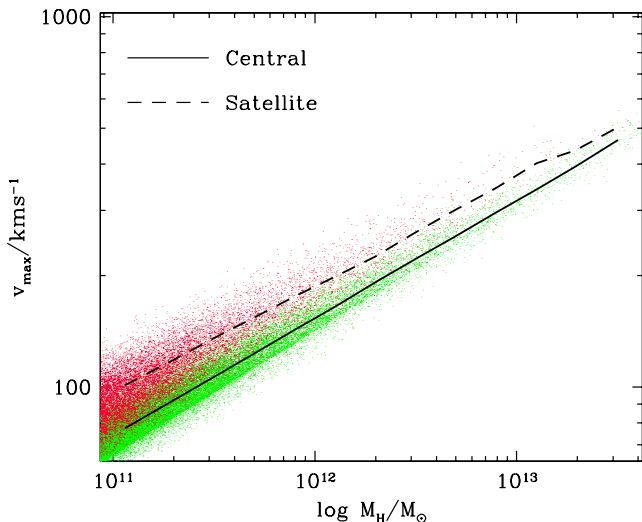
Figure 9. The maximum of the circular velocity profile, v_{\max} , versus the halo mass, M_{\text{H}} ; both measured at infall for subhaloes and at z = 0 for independent haloes. Each green point represents a central galaxy and each red point represents a satellite galaxy. The solid and dashed curves show the mean v_{\max} in bins of M_{\text{H}} for central and satellite galaxies, respectively.
