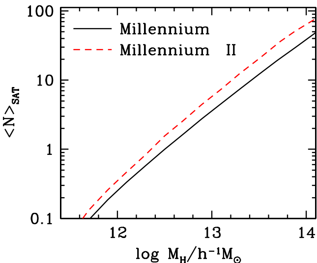
Figure 1. Mean number of SHAM-selected subhaloes per halo as a function of parent halo mass at z = 0 . Subhaloes above an infall mass threshold of 8.6 \times 10^{10} h^{-1} M_\odot are selected which corresponds to 100 times the particle mass in the MS.
