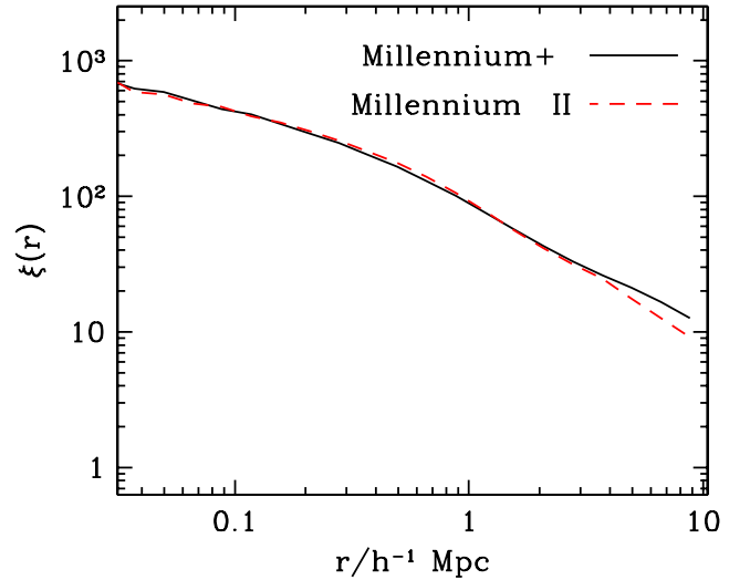
Figure 2. Two-point correlation function of z = 0 subhaloes that are above an infall mass threshold. In the MS-II, we only include subhaloes identified at z = 0 , while in the MS, we add a fraction of disrupted subhaloes to those identified at z = 0 so that we match the mean number of subhaloes per parent halo as a function of parent halo mass in MS-II (see Fig. 1).
