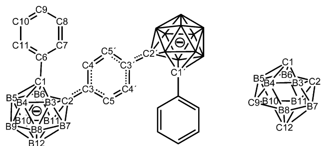
Scheme 2. Generic structures for [3]^{2-} and [4]^{2-} (left) and 5 (right) with atom numbering. The \text{Me}_3\text{Si} groups attached to the carbon atoms in 5 are omitted for clarity.
