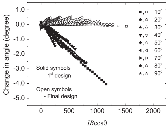
FIG. 4. Data from Fig. 3 replotted as the change in the angle during the J_c measurement as a function of the product of the current ( I ), the applied magnetic field ( B ), and the cosine of the instantaneous angle between magnetic field and the sample's surface at different starting angles.
