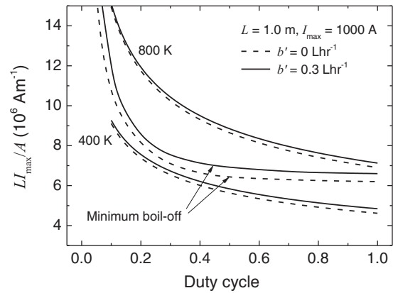
FIG. 13. Calculated optimum shape factors ( LI_{\max}/A ) of a current lead for critical current measurements as a function of duty cycle for a static boil-off ( b' ) of 0 and 0.3 \text{Lhr}^{-1} from Eq. (6) where the current-lead length is 1.0 m and the maximum current 1000 A. One data pair describe optimum conditions for the minimum average helium boil-off and the other two pairs show conditions when the maximum temperature of the current lead is the limiting factor, fixed at 400 K and 800 K.
