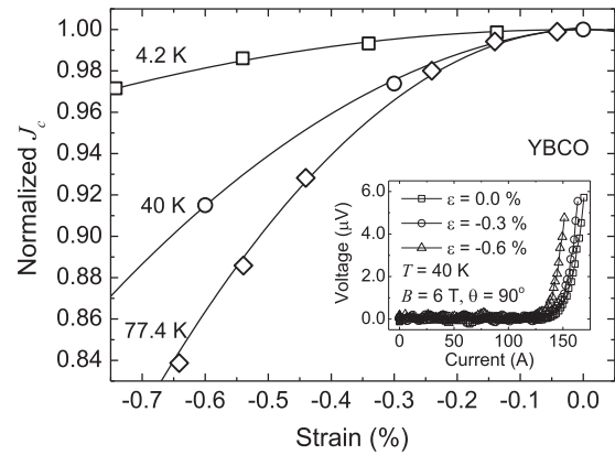
FIG. 24. Normalized critical current density of YBCO tapes as a function of strain at 4.2 K, 40 K, and 77.4 K and 6 T. The inset shows voltage-current characteristics of a YBCO tape at 40 K as a function of applied strain with the magnetic field applied normal to the tape surface.
