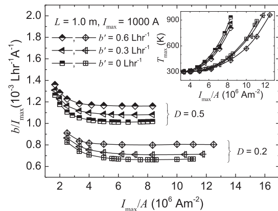
FIG. 11. Calculated average helium boil-off per unit current ( b/I_{\max} ) for two vapour-cooled brass current leads and maximum temperature of the current leads ( T_{\max} —shown inset), as a function of the ratio between maximum current and cross-sectional area ( I_{\max}/A ) of each lead with and without static or sample boil-off. The length of all current leads is 1.0 m. The maximum current investigated was 1000 A.
