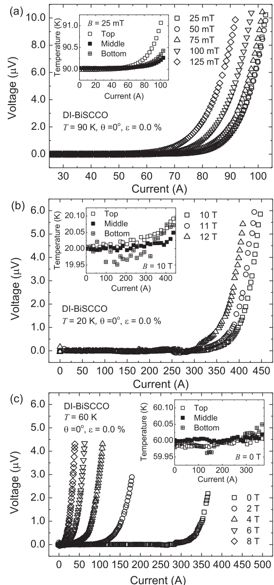
FIG. 16. (a) Voltage-current characteristics of a DI-BiSCCO tape at 90 K, measured as a function of applied magnetic field parallel to the tape surface for measurements in liquid nitrogen. The inset shows the temperature rising during the transition for the data taken at 25 mT where the critical current is 88 A at 100 \mu\text{V m}^{-1} . \Delta T across the voltage taps is 130 mK. (b) and (c) Voltage-current characteristics of the same sample at 20 K and 60 K as a function of applied magnetic field parallel to the tape surface for measurements in liquid helium. The insets show the temperature rising during the transition for data taken at 10 T at 20 K and 0 T at 60 K where the critical currents were 398 A and 352 A, respectively. In both cases, \Delta T across the voltage taps is \sim 30 mK.
