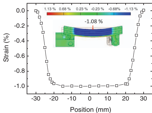
FIG. 20. Computational data of the strain homogeneity on the top surface of the 2.5-mm-thick springboard-shaped sample holder with an applied strain of -1.08\% . The inset shows a colour plot of the data from finite element analysis.
