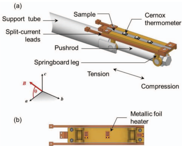
FIG. 18. (a) Diagram of the springboard-shaped sample holder and thermometry. (b) Metallic foil heaters underneath the sample holder.
