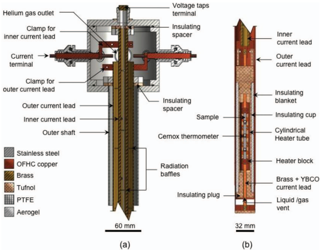
FIG. 1. Diagram of the J_c(B, T, \theta) probe (a) the top part of the probe including cylindrical current lead tubes and (b) the final design of the variable-temperature cup and insulating plug and vent.
