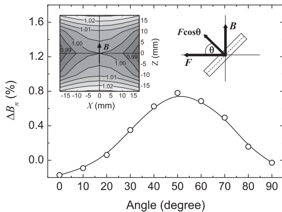
FIG. 5. Change in the normal field component at the sample when the current is at 80 A as a function of the starting angle between magnetic field and the sample's surface for the J_c measurements in this work. The inset shows the normalized magnetic field profile of Durham's split-pair horizontal magnet along the x - z plane which is the plane of the sample's cross-section. Movement of the sample (i.e., change in the normal field component) is attributed to effects of the normal force component ( F\cos\theta ).
