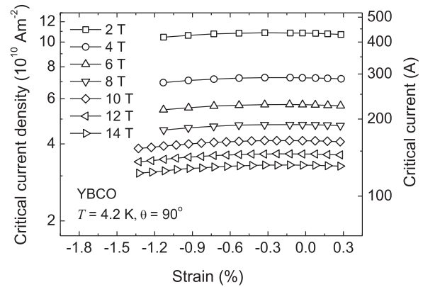
FIG. 21. Critical current density of a YBCO tape at 4.2 K as a function of applied strain for different magnetic fields normal to the tape surface. 4
