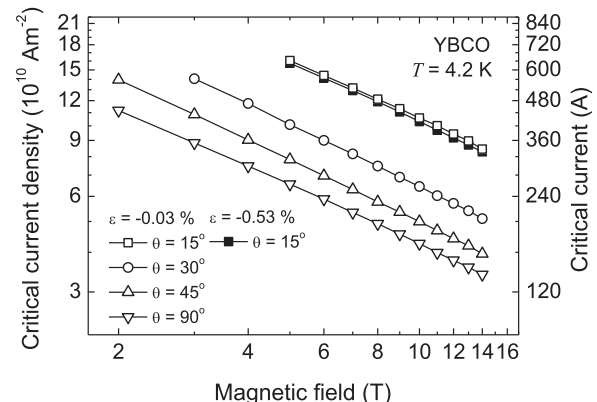
FIG. 22. Critical current density of a YBCO tape at 4.2 K as a function of applied magnetic field for different strains and angles between the magnetic field and the tape surface. 4
