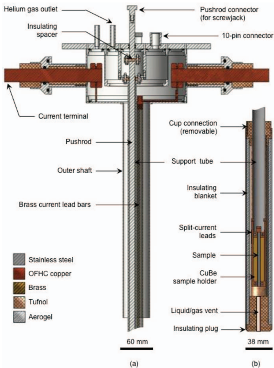
FIG. 17. Diagram of J_c(B, T, \theta, \varepsilon) probe (a) the top part of the probe including a stack of brass current lead bars and (b) the variable-temperature cup, insulating plug and vent.
