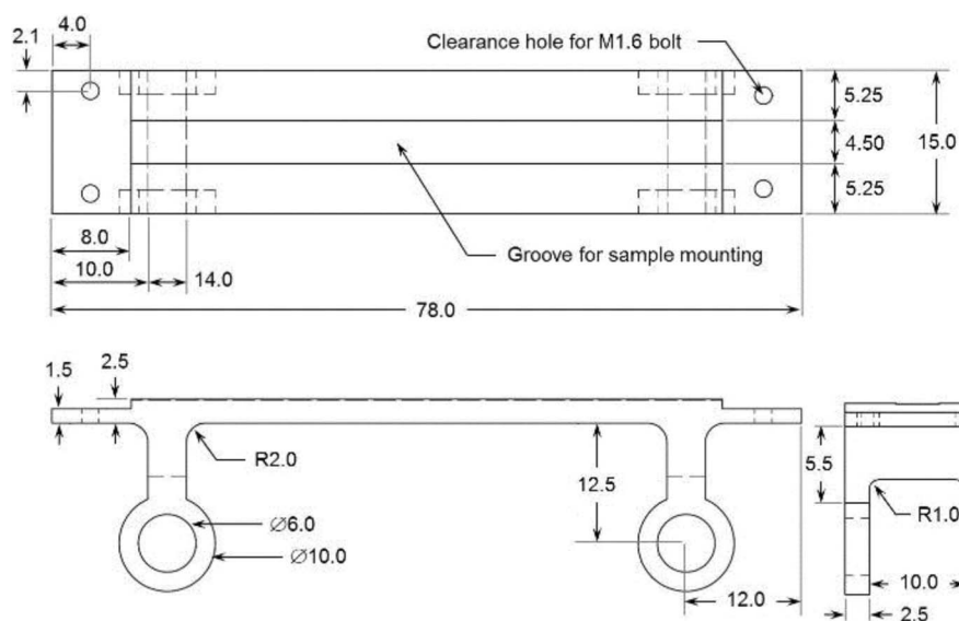
FIG. 19. Technical drawings of the springboard-shaped sample holder.
