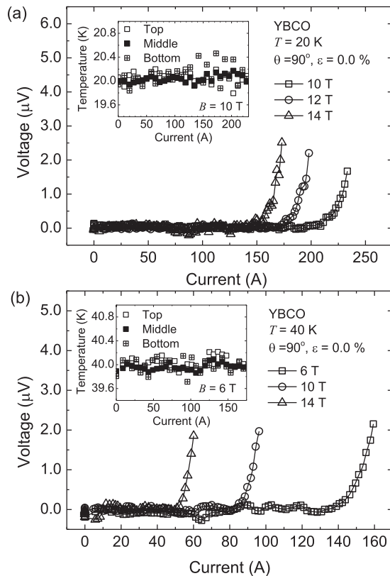
FIG. 23. (a) Voltage-current characteristics of a YBCO tape at 20 K, measured as a function of applied magnetic field normal to the tape surface for measurements in liquid helium. (b) Similar plots at 40 K. The insets show the temperature during the transition for data taken at 10 T at 20 K and 6 T at 40 K where the critical currents at 100 \mu\text{V m}^{-1} were 229 A and 153 A, respectively. In both cases, no systematic temperature increase was observed. The temperature variation was about \pm 150 mK.
