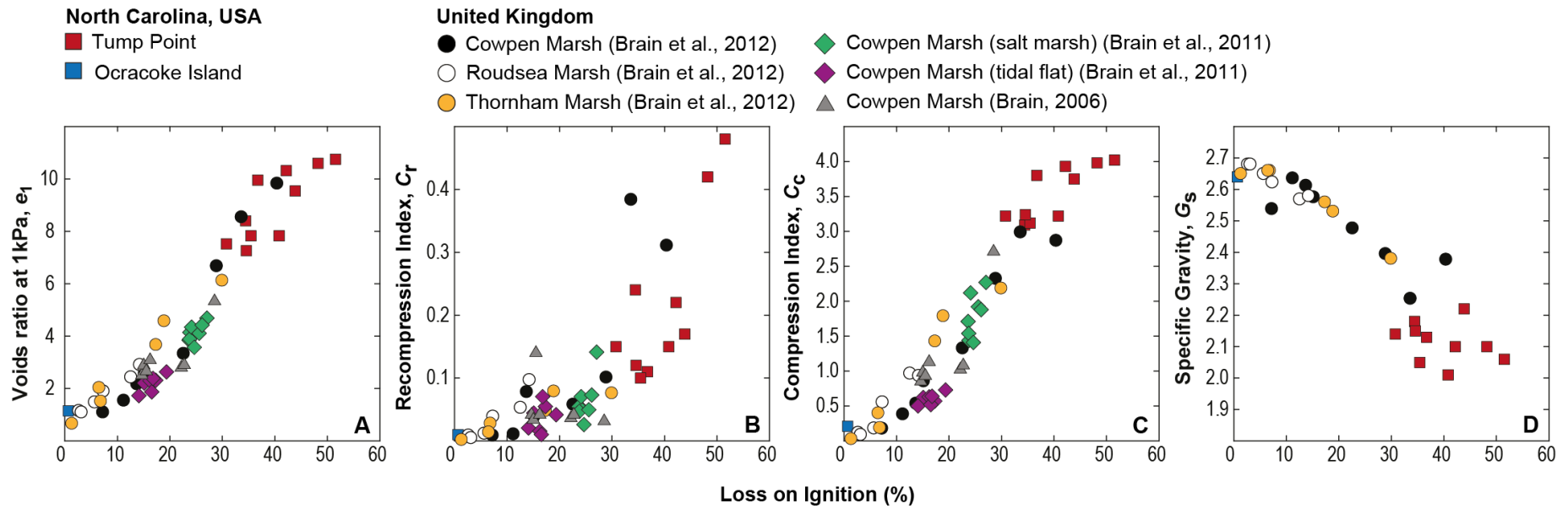
Figure 4. Observed relationships between geotechnical (A – C) and physical properties (D) of salt-marsh sediments used for model calibration.
