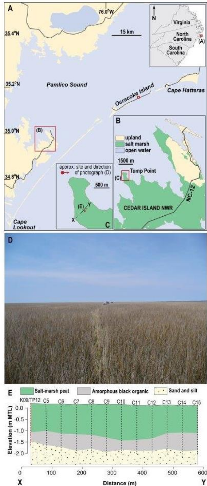
Figure 1. (A - C) Locations of study sites at Tump Point and Ocracoke Island, North Carolina, USA. (D) Photograph of the flat, extensive and ecologically homogeneous salt-marsh platform at Tump Point. Approximate location and direction of view of the photograph are displayed in (C). (E) Simplified stratigraphy underlying the Tump Point site (adapted from Kemp et al., 2009).
