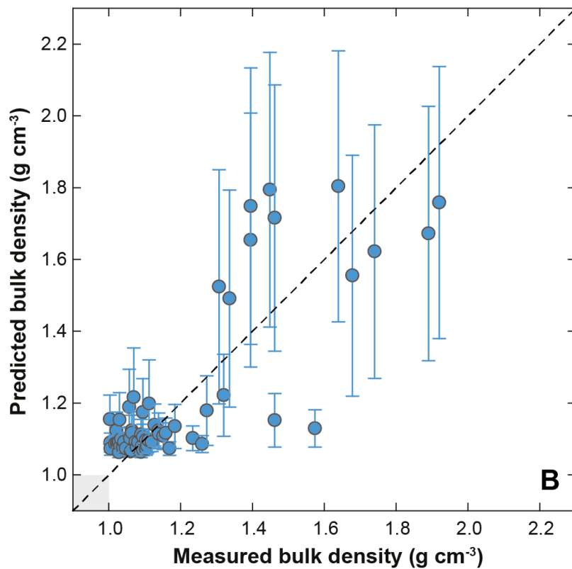
Figure 5. Plots of model-predicted against observed bulk density for the Tump Point core. (A) Full dataset. (B) Data points with observed bulk density < 1 \text{ g cm}^{-3} (i.e. unsaturated sediments) removed. Error bars for values of predicted bulk density represent the standard deviation of the mean of 1000 model runs.
