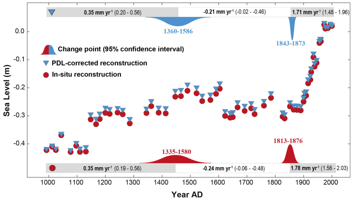
Figure 6. Reconstructed sea-level changes at Tump Point following correction for land-level change ( 0.9 \text{ mm yr}^{-1} ). An error-in-variables changepoint model identified persistent sea-level trends for the in situ (red circles) and decompacted (blue triangles) reconstructions. For clarity, reconstructions are presented as estimate mid points without vertical or temporal uncertainties (see Kemp et al., 2011).
