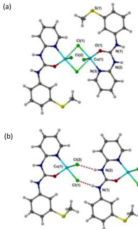
Fig. 3. (a) Dimeric structure of \{[Cu(L)(\mu-Cl)Cl]_2\} ( 1 ) – long axial Cu–Cl interactions shown as dotted lines. (b) R_2^2(8) hydrogen bond motif in 1 (one half of the chloride-bridged dimer is shown for clarity). Selected distances (Å): N(1)\cdots Cl(1) 3.156(6), N(2)\cdots Cl(2) 3.371(6).
