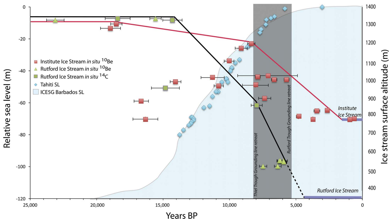
Fig. 4. Reconstructed ice stream trajectories over the last 25 000 years from terrestrial cosmogenic nuclides in glacially transported erratics ( in situ ^{14}\text{C} and ^{10}\text{Be} \pm 1 standard deviation). The profiles of the Rutford and Institute ice streams are shown in green and red, respectively. The grey column defines the timing of inner continental shelf deglaciation of the Thiel Trough and the Rutford Trough, based upon the available calibrated marine ^{14}\text{C} constraints (Hillenbrand et al. 2012, 2014), reflecting the proposed period of ice stream capture of the Institute Ice Stream by the Thiel Trough. For comparison, global relative sea level rise reconstructed from Tahiti (Bard et al. 1996, Bard 2003) and Barbados (Peltier & Fairbanks 2006) are plotted.
