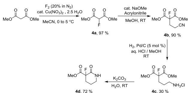
Scheme 4. Initial unoptimised synthesis of racemic 4a-d .
