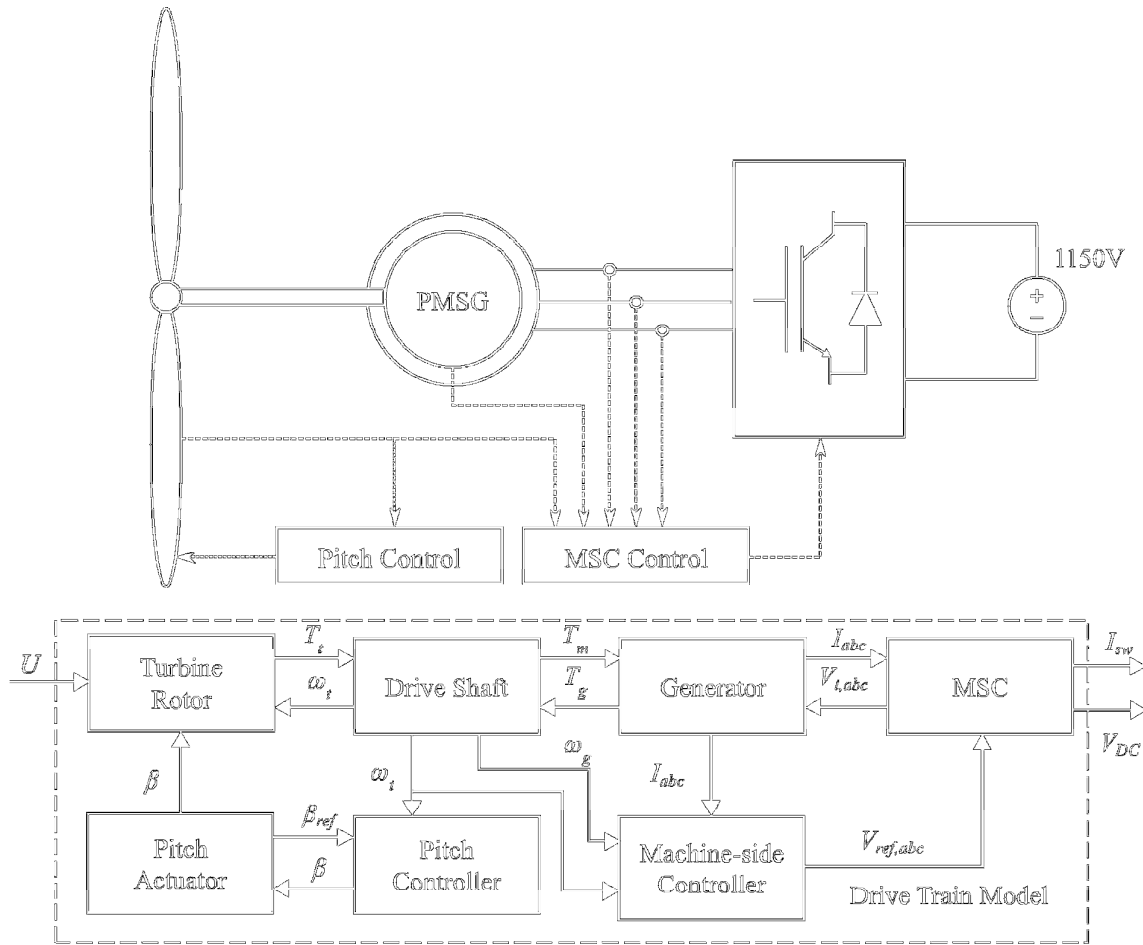
Fig. 3. Drive train model summary
