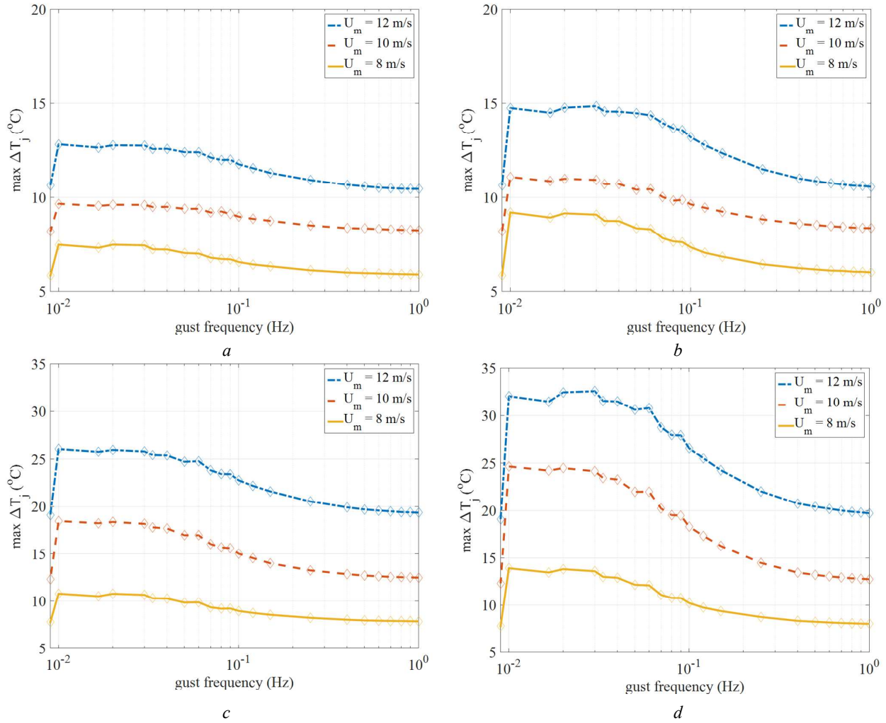
Fig. 8. \max \Delta T_j over varying mean wind speeds ( U_m ) and square gust frequencies for:
