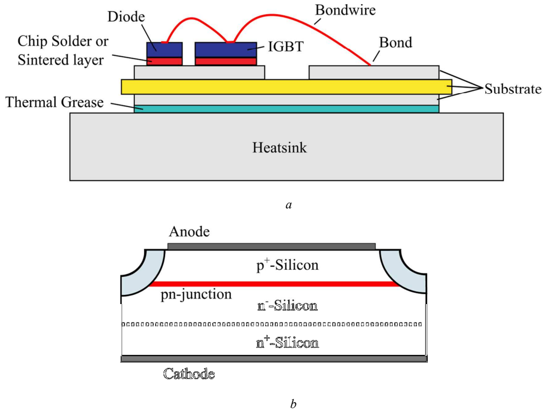
Fig. 1: Chip layout and packaging for typical power module devices. Figures adapted from [6]
