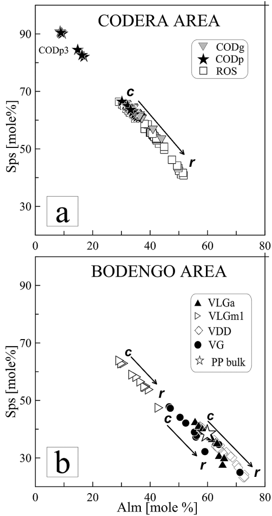
FIG. 11. Almandine (Alm) versus spessartine (Sps) component plot illustrating the composition of garnet from the Codera and Bodengo areas. Garnet from the Codera area is predominantly spessartine (Sps>50%), with minor almandine rims. The highest spessartine content (80–90%) is from garnet of the phosphate-bearing dike of the Codera area (CODp). Garnet from the Bodengo area is typically almandine (Alm>50 %), with the only exception being garnet from the monazite-bearing dike of the Leggia Valley (VLGm), whose composition overlaps garnet from the Codera area. Arrows indicate core (c) to rim (r) compositional trends.
