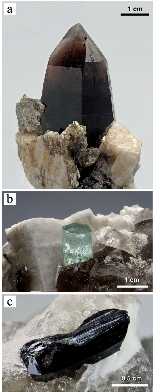
FIG. 7. Pegmatite minerals from miarolitic cavities of the Bodengo area. (a) Smoky quartz with microcline and muscovite. (b) Terminated gem-quality beryl (aquamarine). (c) Twinned crystal of wodginite.
