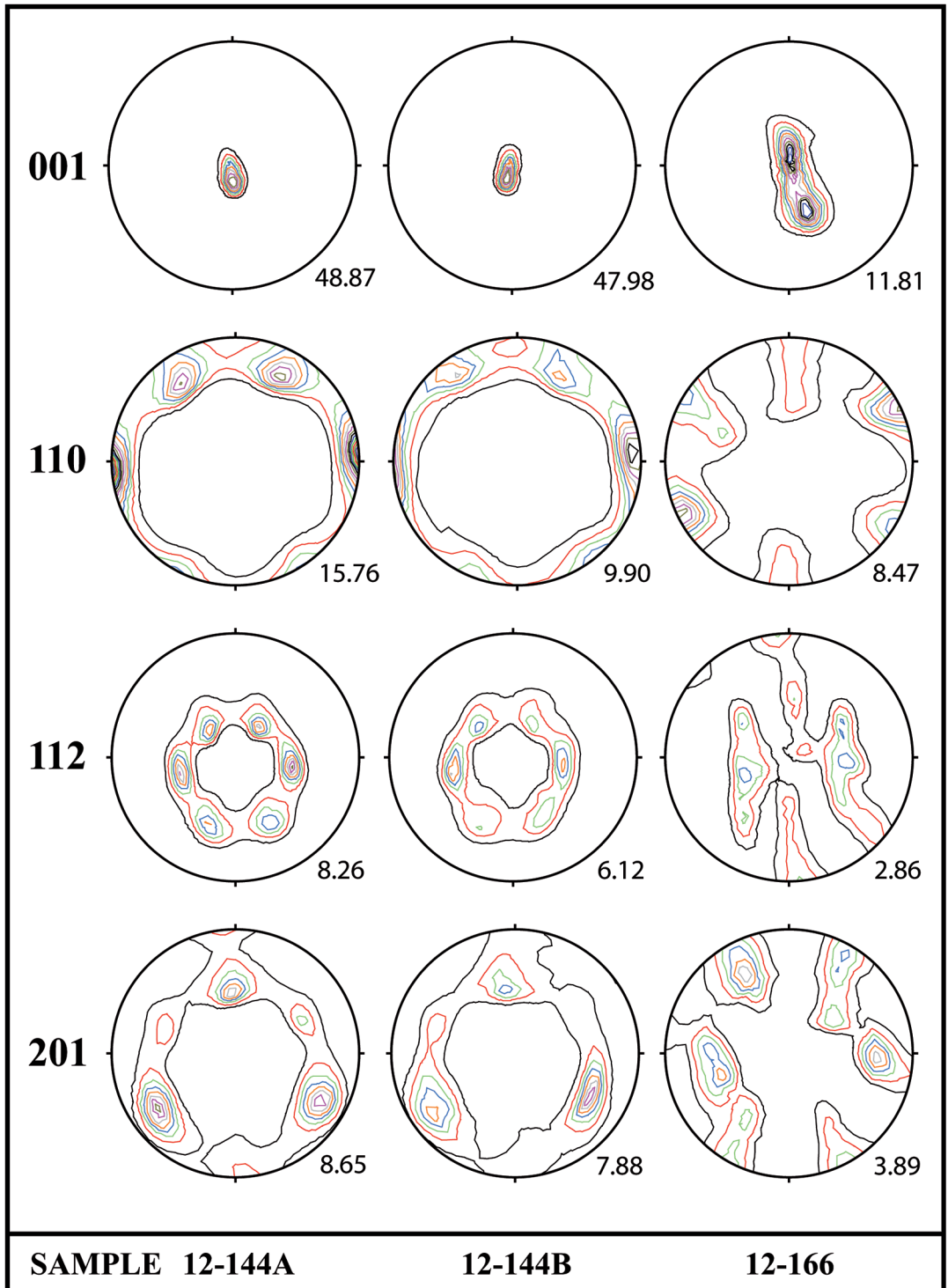
FIG. 9. Plots (upper hemisphere, equal area) of (001) ( c axis), (110) ( \langle a \rangle axis), (112), and (201) axes of quartz mylonites of the Codera area determined by texture goniometry. The plots are cumulative and the total investigated area in each sample is 2 \text{ cm}^2 .
