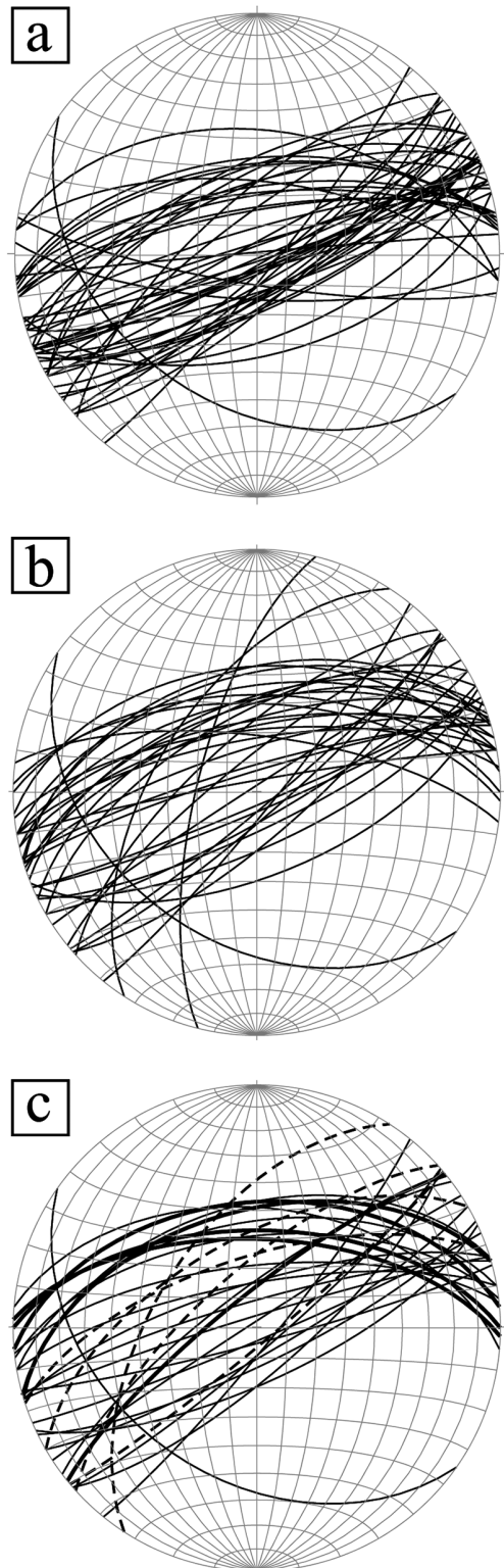
FIG. 4. Stereographic plots (lower hemisphere, equal area) of the orientations of the pegmatite dikes (a), mylonites (b), and ductile deformed dikes and veins (c) from the upper eastern Codera valley. In (c) the thin lines represent pegmatites, thick lines are leucocratic (microgranite) dikes, and dashed lines indicate quartz veins.
