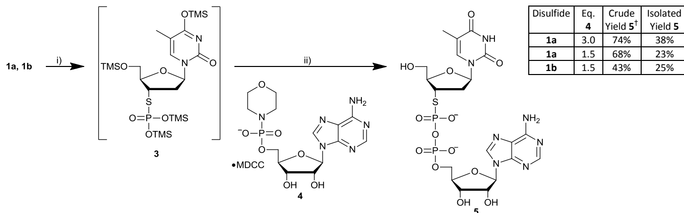
Scheme. Synthesis of dTSPpA. Reagents and conditions. (i) (\text{TMSO})_3\text{P} , BTMSA, \text{CHCl}_3 , RT, 30 min; (ii) a) 4 , tetrazole, \text{MgCl}_2 \cdot 6\text{H}_2\text{O} , \text{H}_2\text{O} , LAG, 30 Hz, 90 min, b) \text{H}_2\text{O} , \text{CH}_3\text{OH} , \text{CH}_3\text{CN} (from 1b ); or \text{H}_2\text{O} (from 1b ). Key. MDCC = 4-morpholine- N,N' -dicyclohexylcarboxamidinium; † calculated using integration of the \beta -phosphoryl resonance (based upon 100% efficient M-A reaction).
