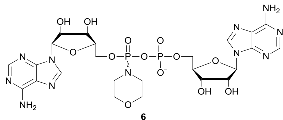
Figure 4. Homocoupled AMP-morpholidate side-product (Ap(M)pA).
