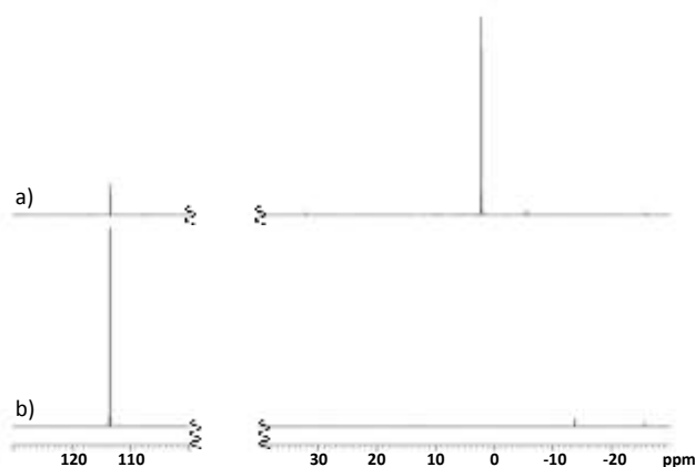
Figure 2. 31 P NMR spectra of: a) 63 mM (\text{TMSO})_3\text{P} (1.1 eq.) and disulfide 1a in 4:1 \text{CHCl}_3 :BTMSA after 30 min at room temperature; or b) 63 mM (\text{TMSO})_3\text{P} in 4:1 \text{CHCl}_3 :BTMSA.
