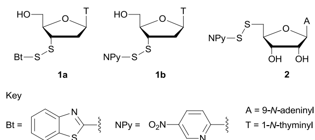
Figure 1. Activated disulfide derivatives used as substrates in directed Michaelis-Arbuzov reactions.
