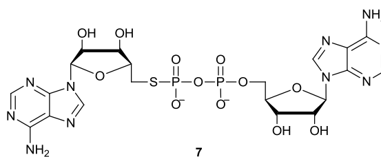
Figure 5. Pyrophosphorothiolate-linked product derived from 5'-thioadenosine (dASppA).
