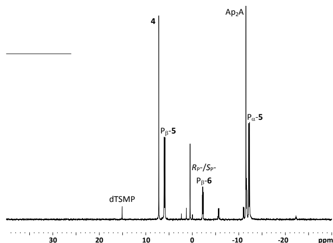
Figure 3. ^{31}\text{P} NMR spectrum of crude ball milling reaction mixture following hydrolysis and phosphate coupling of the putative persilylated M-A product 3 in the presence of 3 eq. AMP-morpholidate ( 4 ).
