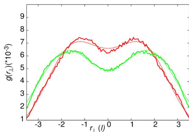
Fig 4 g(r_{\perp}) for the intense local peak centred at r_{\parallel} = 3.54 for core-core distances of separation. Green line – 50 wt% results, red line – 25 wt% results. The gaussian fits use the form of equation 7, with the parameters a_1 = 3.96373 \times 10^{-4} , c_1 = 1.0 , a_2 = 4.92693 \times 10^{-4} , c_2 = 2.5 (25wt%) and a_1 = 6.26241 \times 10^{-4} , c_1 = 1.5 , a_2 = 3.16987 \times 10^{-5} , c_2 = 0.749 (50 wt%).
