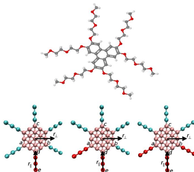
Fig. 1 Top – molecular structure of TP6EO2M. Bottom – model 1 (left), model 2 (centre) and model 3 (right). The sites labelled a , b and c are used in the application of a pseudo-magnetic field. The sites labelled d and e are used, in conjunction with the plane of sites a , b and c , to define the parallel, r_{\parallel} and perpendicular directions, r_{\perp} , (shown with arrows).
