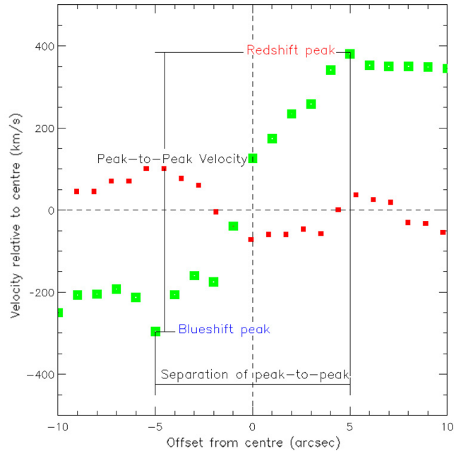
Figure 10. Two examples of a velocity profiles taken from Hydra-A (large green points) and NGC 5044 (small red points). These profiled were used to calculate the peak-to-peak velocity within each system. The contrast of these two objects shows how the peak-to-peak was clear in some objects (such as Hydra-A) while being much more difficult to constrain in others (such as NGC 5044). The blueshift peak and redshift peak are labelled and the peak-to-peak velocity and peak-to-peak separation are indicated for Hydra-A.
