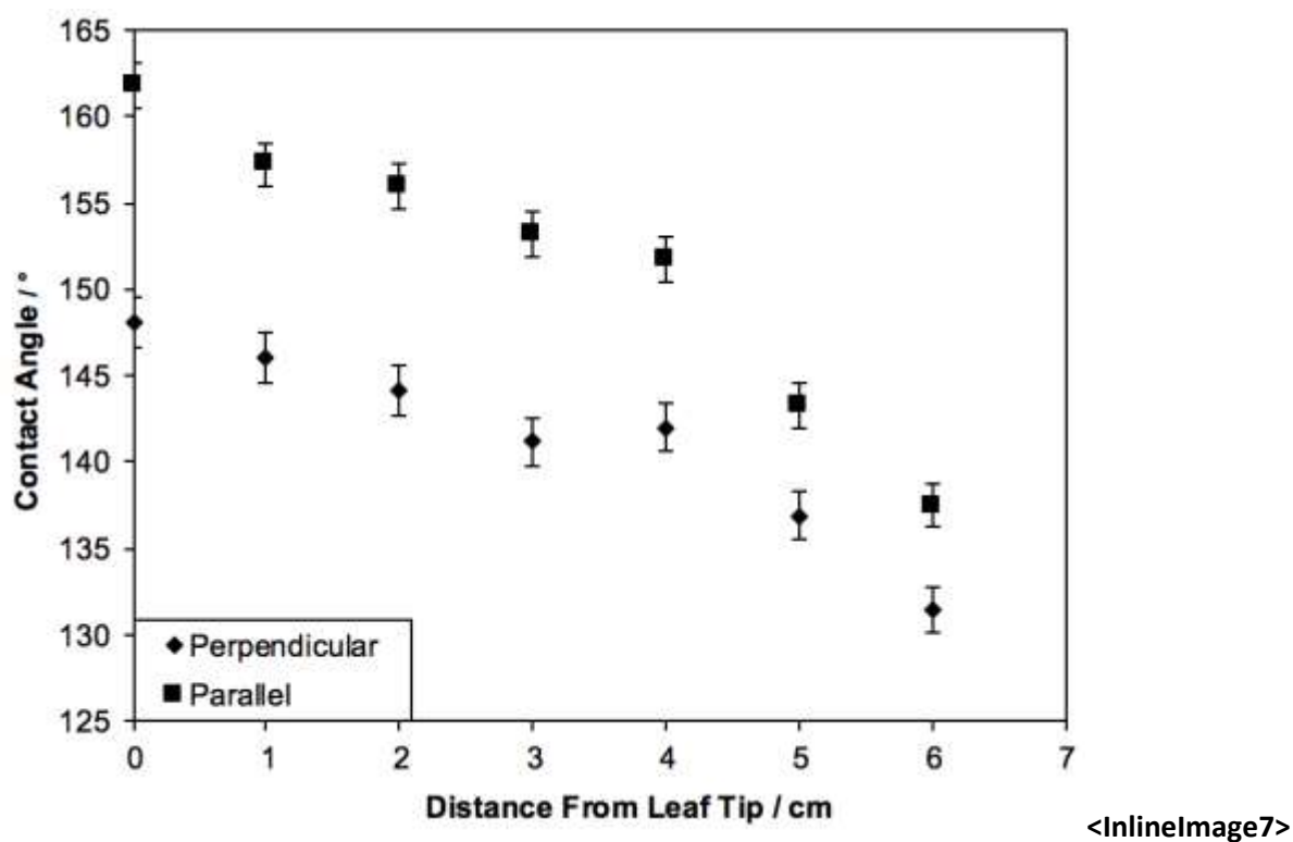
Figure 3: Water contact angle values viewed parallel (along) and perpendicular to the length of Eremopyrum orientale plant adaxial leaf surface as a function of longitudinal distance from the leaf tip (total length 6 cm).
