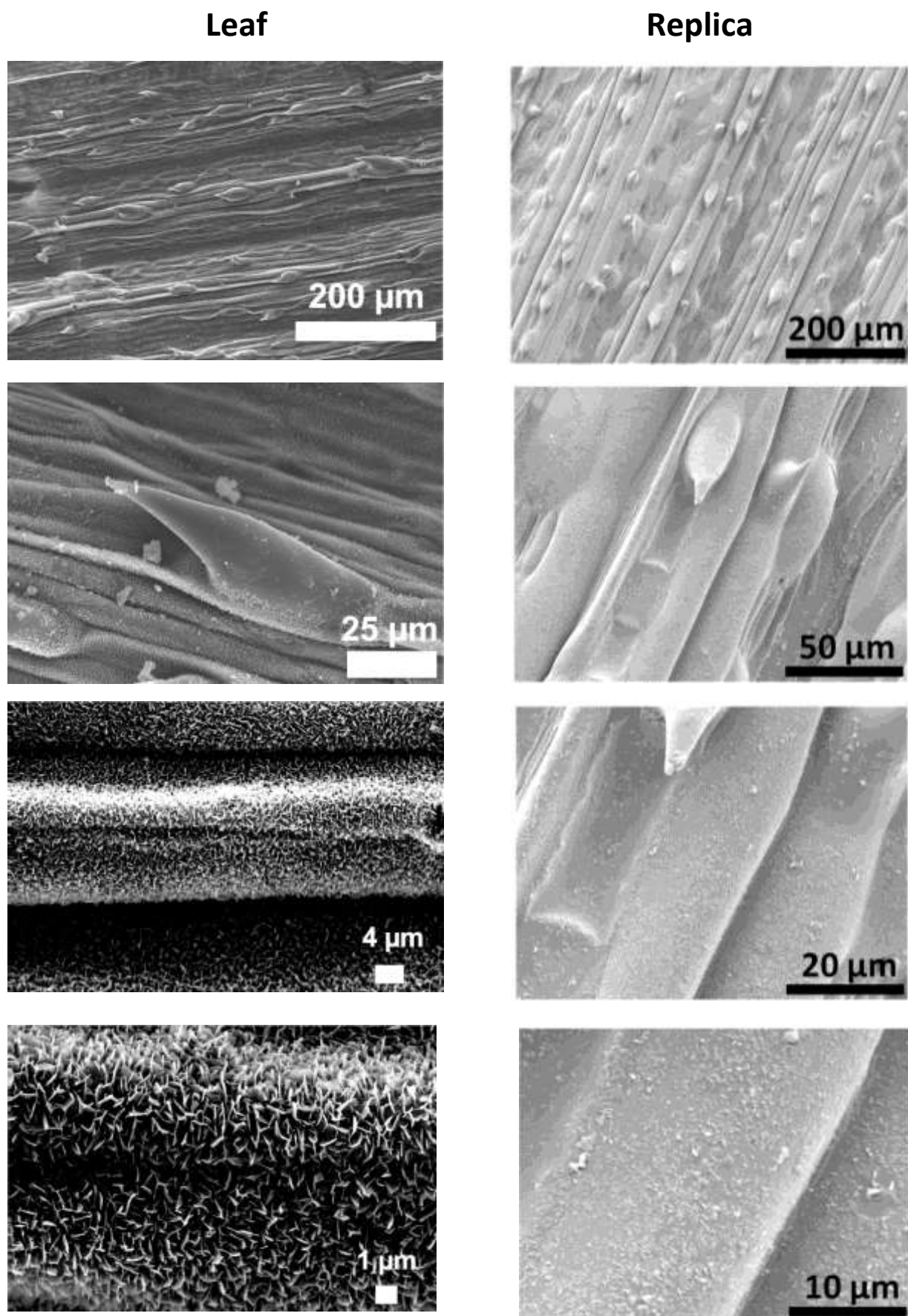
Figure 4: SEM images of Eremopyrum orientale adaxial leaf middle region and replica.
