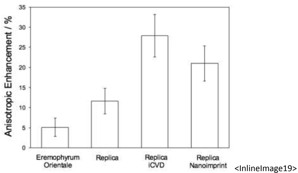
Figure 6: Anisotropic (directional) enhancement of steady state mist collection efficiencies for micro-scale tilted cones pointing vertically downwards versus upwards for Eremophyrum orientale adaxial leaf, unfunctionalised replica, iCVD functionalised replica, and functional nanoimprint replica, see Supplementary Material Figure S2.
