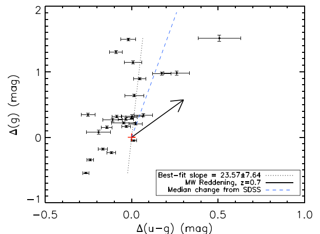
Figure 12. Net colour changes during our period of monitoring. As for Fig. 11, but now for u - g versus \Delta g . The trend line is consistent with no change in colour. Note that the best fit may be not exactly vertical partly as a consequence of forcing the line to pass through the 0,0 point.
