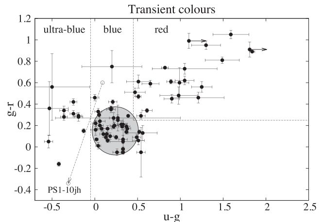
Figure 1. Colours of the PS1 nuclear transients. The horizontal and vertical dashed lines divide the plane into colour classes, as explained in the text. The grey translucent ellipse shows the location of 90 per cent of SDSS spectroscopic quasars (see the text). The points connected by arrows show two versions of PS1-10jh, the TDE candidate from Gezari et al. (2012). The upper circle is the version published by Gezari et al, based on difference imaging; the lower circle is the LT 2 arcsec photometry version, which includes the host galaxy contribution.
