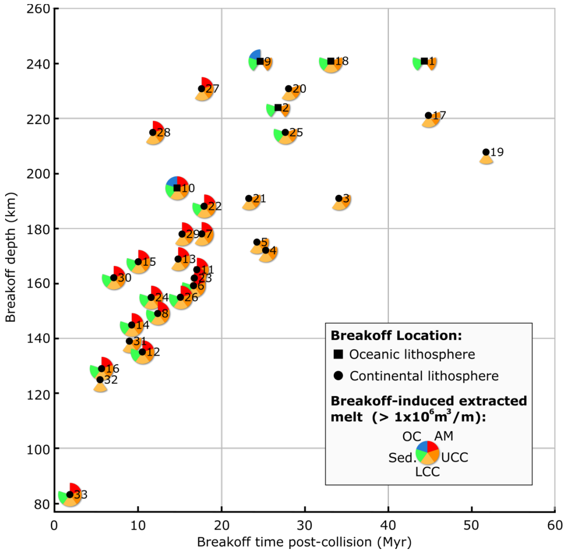
Figure 4 – Breakoff depth versus breakoff time across the parametric study (see Table 3 for details of each model). Models which show melt extraction over 1 \times 10^6 \text{ m}^3/\text{m} as a direct result of breakoff are highlighted for the asthenospheric mantle, upper and lower continental crust, sediments, and oceanic crust. Squares refer to models with breakoff in the oceanic part of the slab and circles indicate breakoff in the continental part of the slab. Models 1-32 are those within the parametric study, whilst Model 33 is an anomalous case, designed to induce very shallow breakoff.
