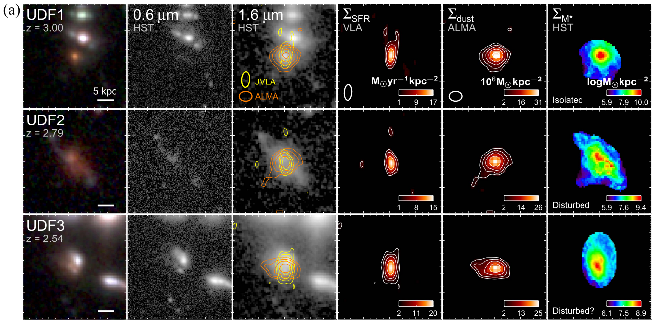
Figure 1. (a) The 11 SFGs detected in both the VLA and ALMA HUDF surveys. From left to right: HST i_{814} - J_{125} - H_{160} color composite; unobscured star formation ( HST /F606W); rest-frame optical morphology ( HST /F160W); star formation rate surface density, \Sigma_{\text{SFR}} (VLA, details in Section 2); dust mass surface density, \Sigma_{\text{dust}} (ALMA, details in Section 3.3); and stellar-mass surface density, \Sigma_{M_*} (from spatially resolved SED fitting using HST images). Each image is 4'' \times 4'' ; north is up, east is on the left. VLA and ALMA synthesized beams are shown in the corresponding columns; the contours are [-3, 3^1, 3^{1.5}, 3^2, \dots] \times \sigma for VLA and [-2.5, 2.5^1, 2.5^{1.5}, 2.5^2, \dots] \times \sigma for ALMA; negative contours are shown as dotted lines. Intense star formation most frequently occurs within the stellar-mass concentration and extends over a large area of the stellar-mass buildup, i.e., galaxy wide. (b) We note that the radio \Sigma_{\text{SFR}} maps for UDF7, 11, and 13 that harbor X-ray-selected AGN with radio emission enhanced more than twice the level of star formation emission (Figure 2, tabulated in Table 1) may contain significant contributions from the AGN and hence are marked as “radio AGN”.
