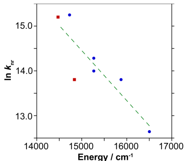
Figure 8. Plot of \ln k_{nr} versus the emission energy as estimated from \lambda_{max} in the solid-state spectra. Data points for phenanthridine complexes are shown as blue circles; quinoline complexes as red squares. The dashed green line is the best linear fit using all data points.
