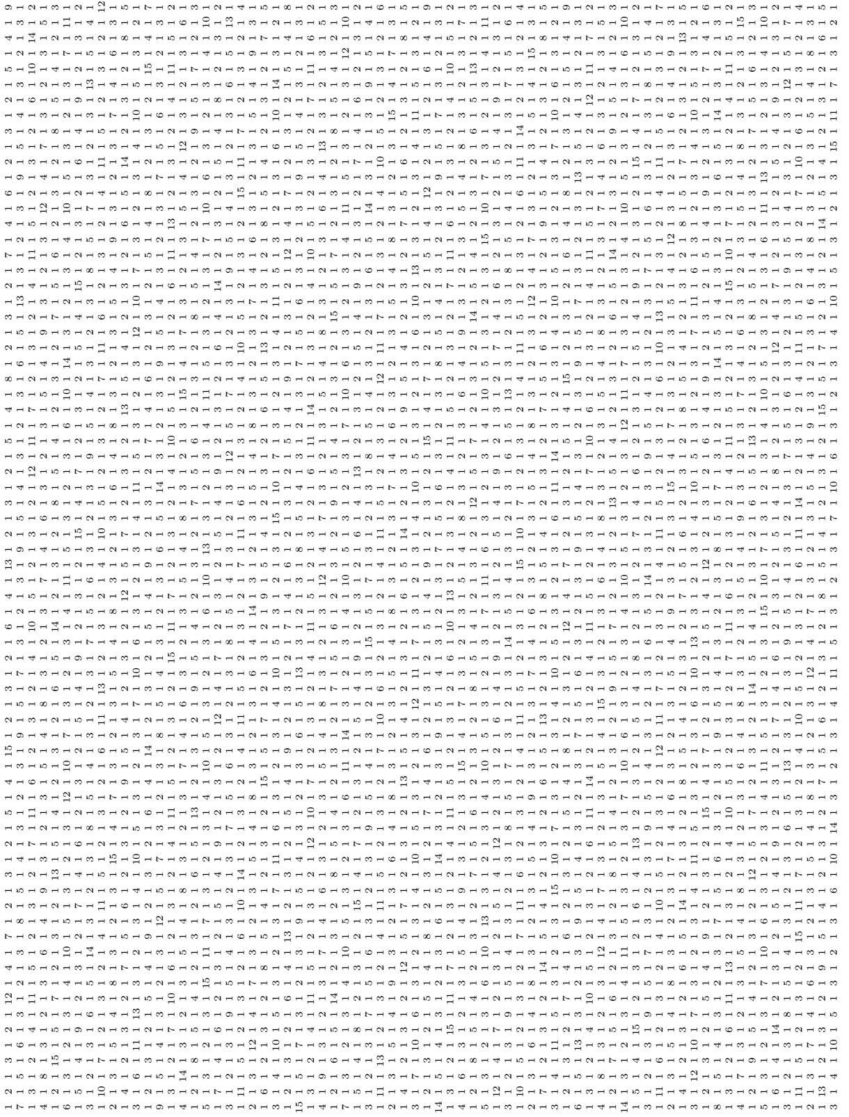
Figure 4: Our 72 \times 72 periodic solution in 15 colours
