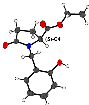
Fig. 3. Molecular structure in the crystals of 6a . The stereocentre at C4 is shown for clarity. Thermal ellipsoids are shown at the 50% probability level.
