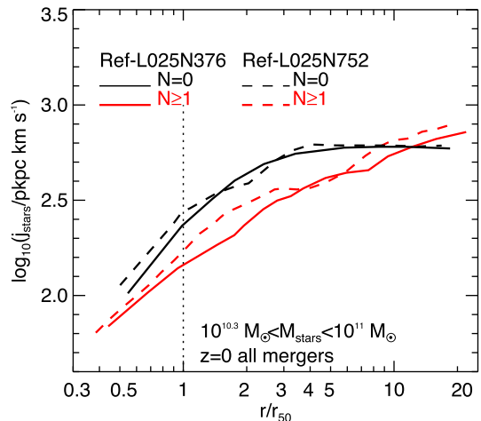
Figure A1. j_{\text{stars}}(r) as a function of r for galaxies with stellar masses in the range 10^{10.3} M_{\odot} < M_{\text{stars}} < 10^{11} M_{\odot} at z = 0 for the Ref-L025N0376 (solid lines) and Ref-L025N0752 (dashed lines) simulations. Lines show the median j_{\text{stars}}(r) . The 16th–84th percentile ranges are similar to those shown in Fig. 7.
