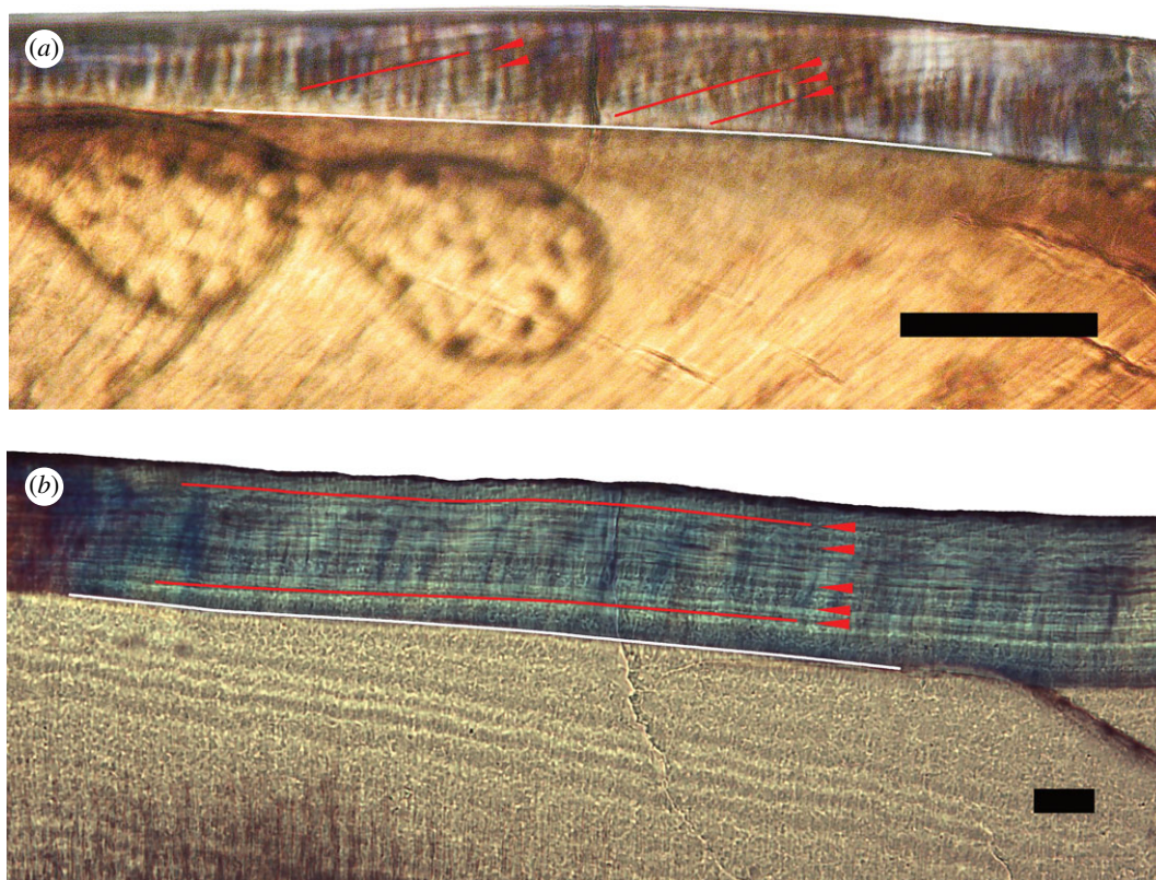
Figure 7. Polarized light microscope images of incremental lines in the enamel of postcanines of the mammaliomorph M. watsoni UMZC 2017.4.1 (a) and the non-probainognathian Diademodon sp. UMZC T.486 (b). Red arrows indicate prominent long-period incremental lines, with the paths of some traced for emphasis. White lines indicate the EDJ. Long-period lines of Morganucodon approach the EDJ at a steeper angle of inclination, indicating more gradual accretion of enamel than in Diademodon , in which enamel is rapidly extended, causing long-period lines to approach the EDJ at a very small angle. Scale bars, 50 \mu\text{m} . Cervix to the left in both images.
