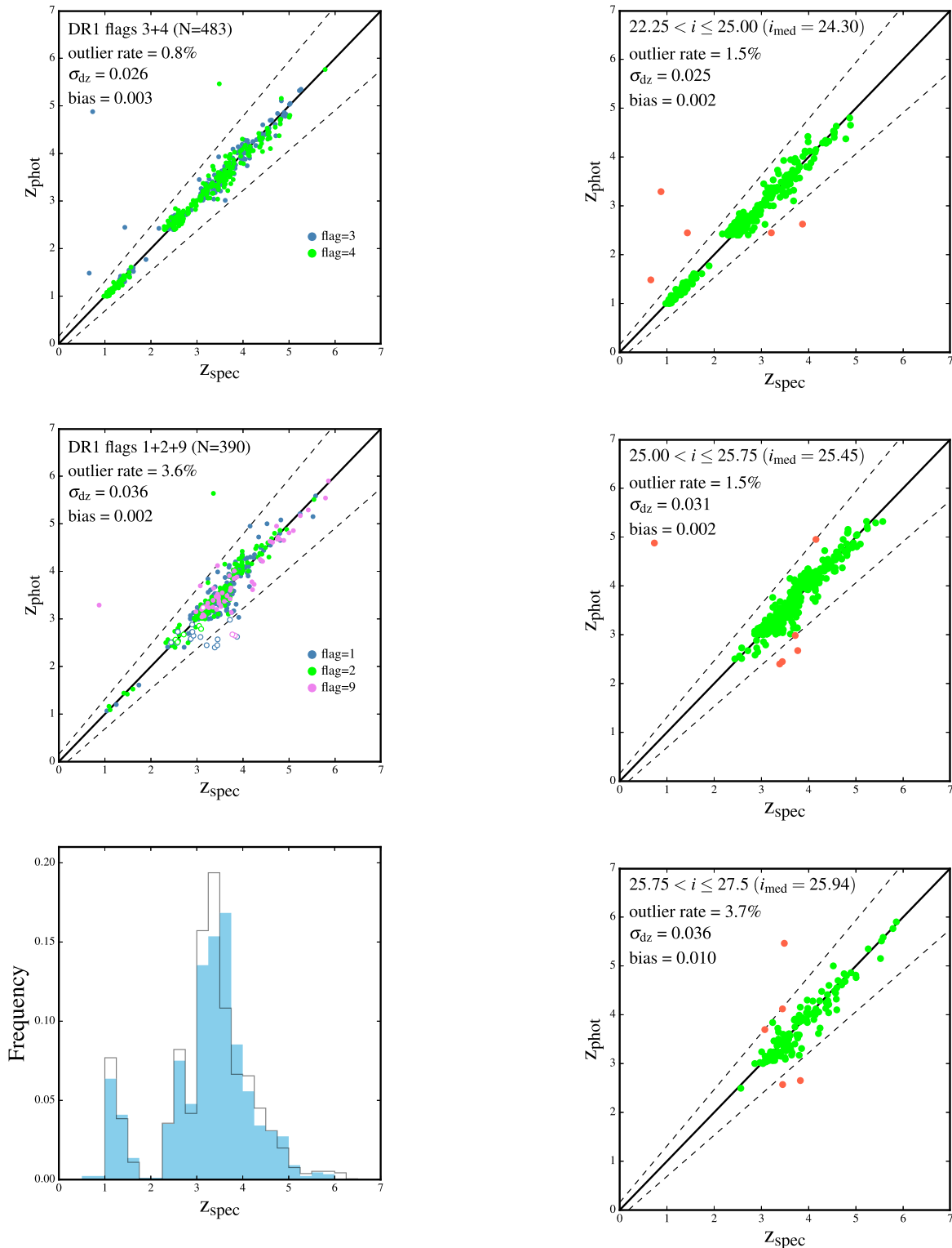
Figure 8. The top panel shows a comparison between the input photometric redshifts and measured spectroscopic redshifts for DR1 galaxies with redshift quality flags 3 and 4. The middle panel is the equivalent plot for DR1 galaxies with redshift quality flags 1, 2, and 9. Those galaxies falling outside the dashed lines are catastrophic outliers with |dz| > 0.15 . In both panels, candidate AGNs and Herschel -detected galaxies are plotted as open symbols. The bottom panel shows a comparison of the spectroscopic redshift distribution of the DR1 galaxies (solid blue histogram) and the photometric redshift distribution of the full VANDELS parent sample (open histogram).
