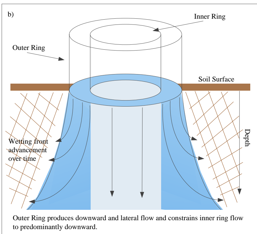
Fig. 1. Descriptions of in situ field permeability principles, a) Guelph Permeameter, b) Double Ring Infiltrometer
