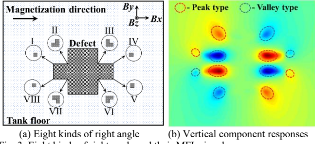
Fig. 3. Eight kinds of right angle and their MFL signal responses.
