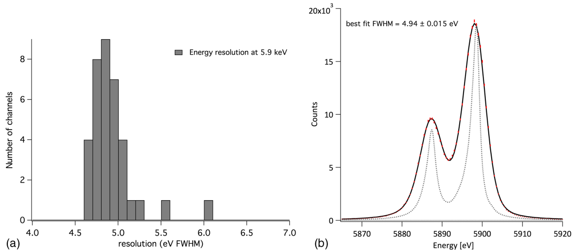
Fig. 6 (a) A histogram of the distribution of resolutions measured across the array. (b) The whole-array spectrum around 5.9 keV. The points are the data, with \sqrt{N} error bars on the counts barely visible. The dark line is the best fit to a model of the natural line shape convolved with Gaussian broadening, and the dashed grey line is the natural line shape.
