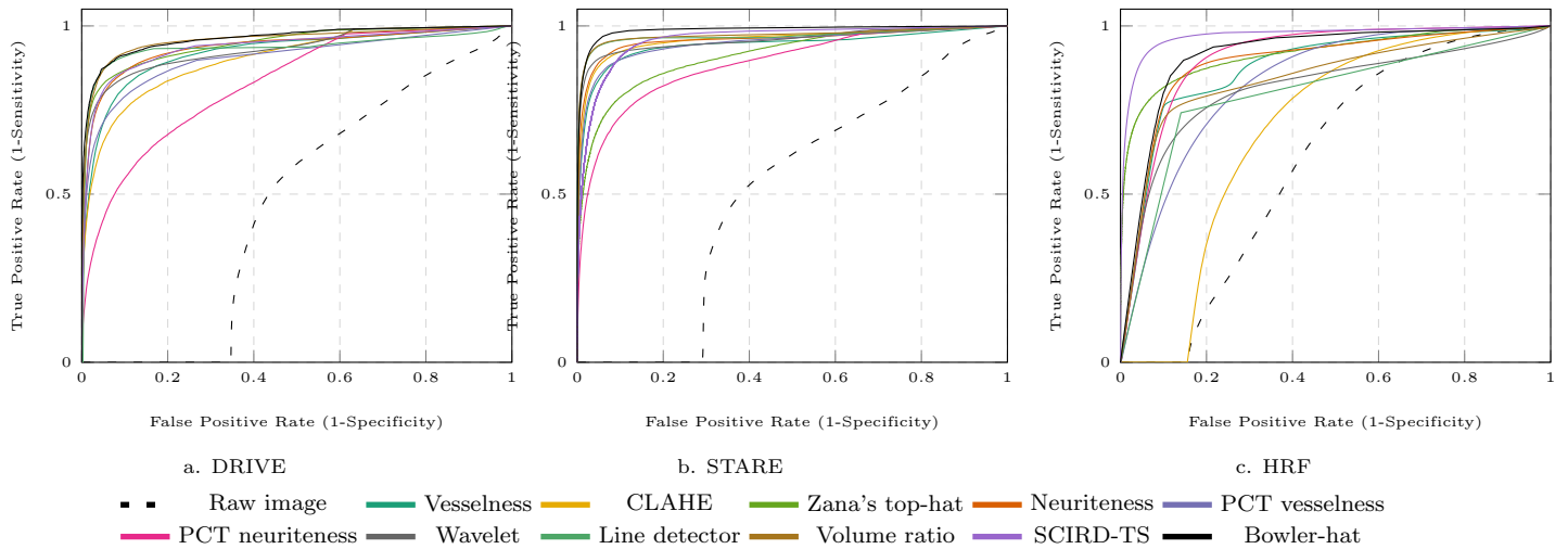
Figure 8: ROC curves calculated for sample images from the (a) DRIVE, (b) STARE, and (c) HRF datasets enhanced by the proposed and the state-of-the-art methods (see legend for colours). Corresponding mean AUC values can be found in Table 1.
