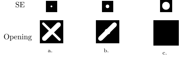
Figure 2: An opening of a simple image with the various size of structuring elements (SE) (the left route in Figure 1). (a) is a result of after a SE smaller than any curvilinear features, (b) is result of after a SE bigger than some curvilinear features but smaller than the other features and (c) is result of after a SE bigger than all curvilinear features in the input image. Reprinted with the permission from [40].
