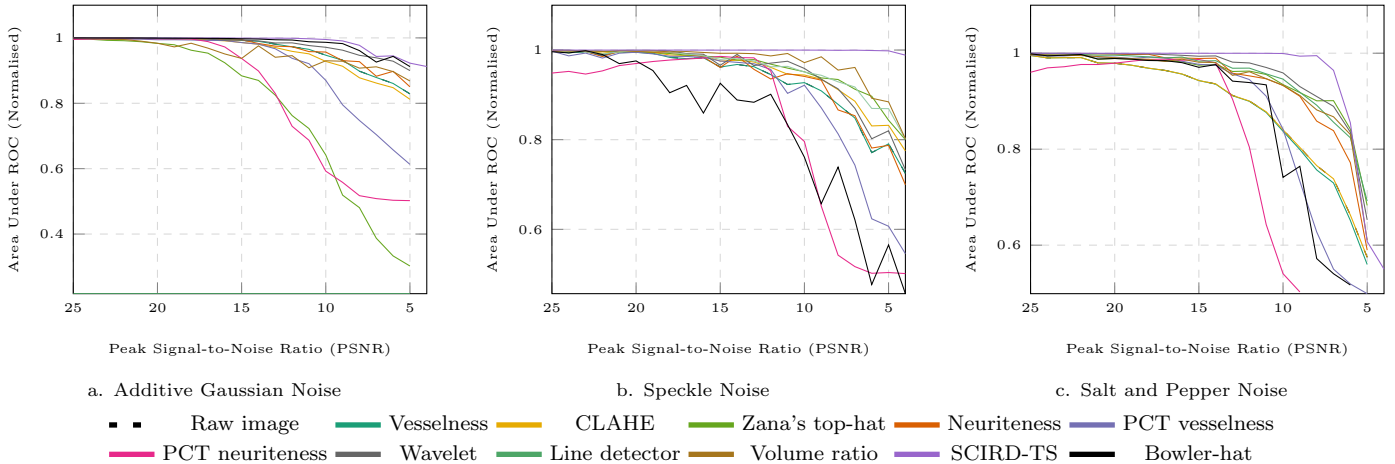
Figure 11: The bowler-hat transform is robust against additive Gaussian noise but susceptible to speckle and salt&pepper. Mean AUC for the input image and the image enhanced by bowler-hat and by the state-of-the-art methods with different peak signal-to-noise ratios (PSNRs) for three different noise types: (a) additive Gaussian noise, (b) multiplicative Gaussian noise, and (c) salt and pepper noise (see legend for colours).
