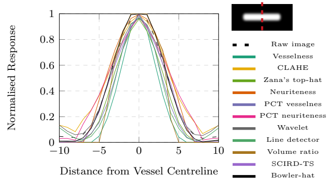
Figure 4: Cross-sectional profiles of a synthetic vessel input image (at the up right side (red, dashed line)) and the input image enhanced with the state-of-the-art (see legend for colours) vessel enhancement methods and the proposed bowler-hat (black, solid line) vessel enhancement method. All the images were normalised such that the brightest pixel in the whole image has a value of 1 and the darkest a value of 0.
