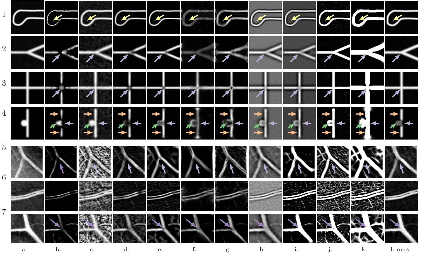
Figure 6: The bowler-hat transform enhances vessels, maintaining junctions and tips while suppressing blobs. A comparison of the enhancement of vessel-like and other structures using the proposed method and the state-of-the-art methods. (a) shows the original images, all vessels have a thickness of 9 pixels and the ‘blob’ in 4 has a diameter of 21 pixels. The first four rows are synthetic images that indicate possible vessel-like structures in biomedical images. The last three rows illustrate vessel-like structures from real biomedical images. Row 5 is a cropped region from the DRIVE dataset, while row 6 is vessel section of the healthy images in the HRF dataset. The last row is another a cropped region from the leaf image [6]. Results for (b) vesselness, (c) CLAHE, (d) Zana’s top-hat, (e) neuriteness, (f) PCT vesselness, (g) PCT neuriteness, (h) wavelet, (i) line detector, (j) volume ratio, (k) SCIRD-TS, and (l) the bowler-hat. Arrows indicate features of interest: vessel structures (yellow arrows), junctions (purple), blob-like features (green), and tips (orange).
