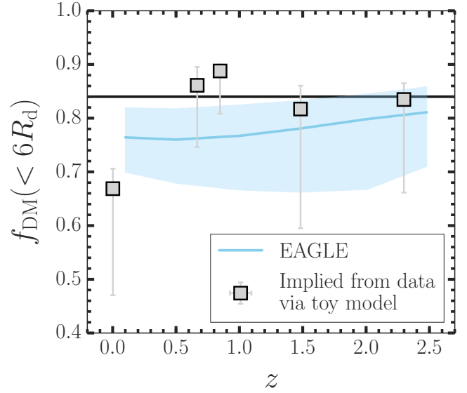
Figure 12. The implied average dark matter fraction ( f_{DM} ) within 6R_d as a function of redshift for our samples, estimated from comparison with a baryonic disk plus dark matter halo toy model. Our best estimate assumes that the baryons in each galaxy are present within a single disk with a single scale radius. The lower error bar reflects the possibility that different baryonic components may have different scale radii, and specifically that a substantial amount of gaseous mass in each galaxy is sufficiently extended such that it has the same dynamical effect as a dark halo within 6R_d . We find no significant evolution in the implied average dark matter fraction of star-forming galaxies since z \approx 2.2 . The blue solid line and shaded region represent respectively the median and the standard deviation of the dark matter fraction measured within 6R_d for massive ( M_*/M_\odot > 10^9 ), star-forming ( > 1M_\odot \text{ yr}^{-1} ) model galaxies in EAGLE (where we linearly interpolate between points to better highlight the general trend). The average trend for model EAGLE galaxies is consistent with our observational, toy model-based estimates. The universal dark matter fraction is indicated with a horizontal line.
