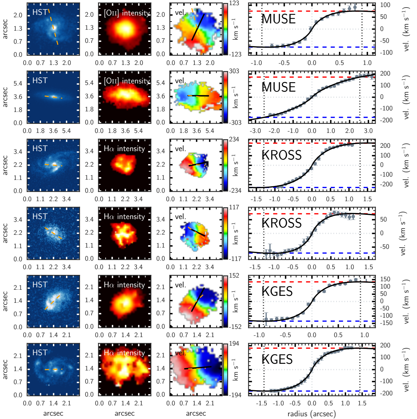
Figure 2. Example data for galaxies in our sample. The panels from left to right are (1) The Hubble Space Telescope broadband image with the morphological position angle (measured from a two dimensional Gaussian fit to the image) overlaid as an orange dashed line. (2) The model H\alpha intensity map constructed by integrating the best fit to the H\alpha emission line in each spaxel. (3) The observed line-of-sight velocity map constructed by plotting in each spaxel the H\alpha peak position from the simultaneous best fit to the H\alpha and [N\ II] triplet – this in velocity space and with respect to the galaxy systemic velocity. We overlay the kinematic position angle (corresponding to the maximum velocity gradient along a “slit” of width equal to half that of the PSF) as a black solid line. We also include the morphological position angle, again as an orange dashed line. (4) The observed rotation curve extracted from a “slit” of width equal to half that of the PSF, in spaxel wide steps. At each radius the observed rotation velocity is taken as the median across the slit. The black solid curve shows the best fit exponential disk model to the data. Black, dotted vertical lines are displayed at \pm 3 times the disk scale radius ( R_d ). We show the observed velocity extracted at \pm 3R_d as the red and blue dashed line, respectively.
