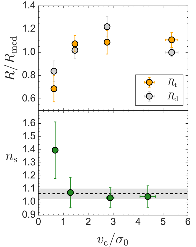
Figure B1. Top: The median size of the KROSS galaxies as a function of v_c/\sigma_0 and with respect to the overall median of the sample. We include the trends for both the dynamical turnover radius measured from the galaxy rotation curves ( R_t ), and the stellar disk-scale radius ( R_d ), measured from broadband imaging. Both measures of size remain approximately constant within uncertainties for v_c/\sigma_0 \gtrsim 1 , but decrease with respect to the overall median of the sample for v_c/\sigma_0 \lesssim 1 . This effect is seen most strongly for the R_t size measurement. Bottom: The median Sérsic index (as measured from H -band HST imaging by van der Wel et al. 2012) as a function of median v_c/\sigma_0 for a sub-set of 102 KROSS galaxies within the CANDELS fields. The black dashed line and grey shaded region represent respectively the median Sérsic index for the total sample and its standard uncertainty. Dispersion-dominated systems ( v_c/\sigma_0 \lesssim 1 ) have a larger median Sérsic index (despite a large associated uncertainty) than that for rotation-dominated systems ( v_c/\sigma_0 \gtrsim 1 ) or for the total sub-set.
