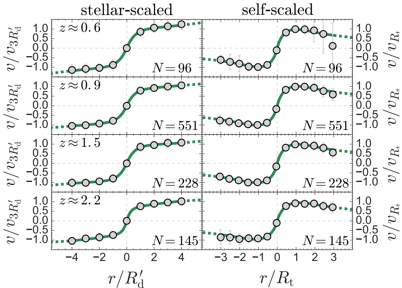
Figure 3. Median stacks of the rotation curves extracted individually from each galaxy in the z \approx 0.6 , z \approx 0.9 , z \approx 1.5 , and z \approx 2.2 samples. For the same data , we employ two normalisation prescriptions. Left column: Median stack normalised by the modified stellar disk-scale radius ( R'_d ) and the velocity at 3R'_d ( v_{3R'_d} ). Right column: Median stack normalised by the galaxy turnover radius ( R_t ) i.e. the rotation curve inflection point) and the velocity at R_t ( v_{R_t} ). For each median rotation curve (grey points), we also plot the best fit exponential disk plus dark halo model (solid green line; the dashed green line represents extrapolation of the same model beyond the extent of the data). The shape of the median average rotation curve for the same galaxies starkly differs depending on the normalisation technique.
