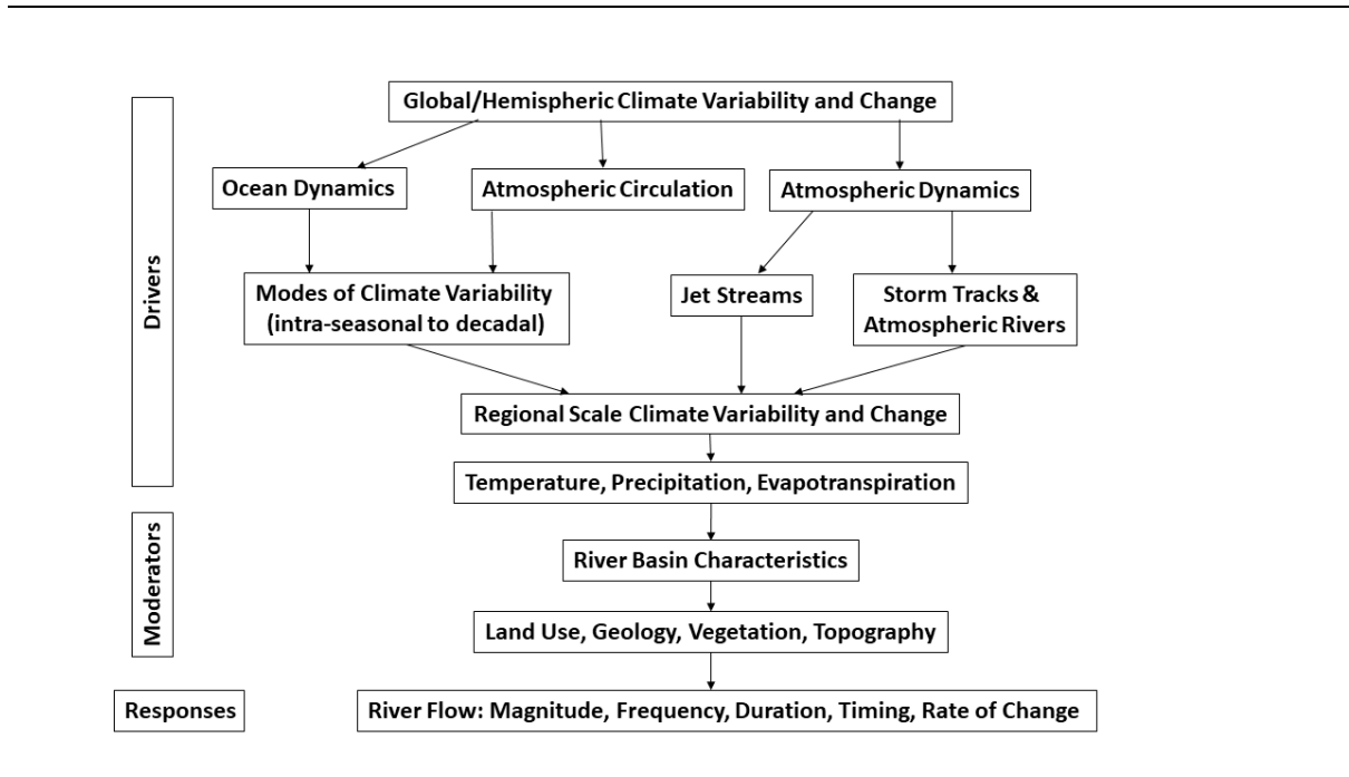
Figure 1: Conceptual model of climate to river basin links, visualising cascade of processes linking a range of atmospheric drivers and river flow response as moderated by river basin characteristics.
