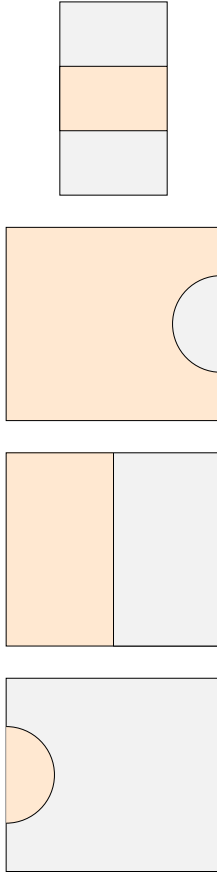
Fig. 4. Equilibrium shapes in any dimensions, depending on the proportion of the lighter versus the heavier fluid: orange stands for the lighter fluid, while gray stands for the heavier fluid
