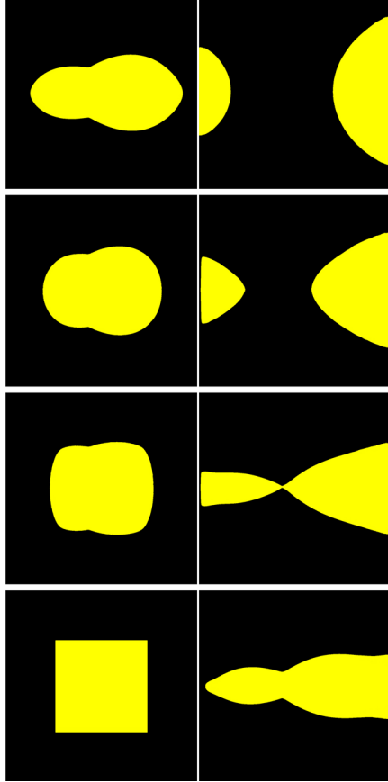
Fig. 3. Numerical simulation of the Muskat problem evolution with a vertical potential that attracts the yellow phase to the top and the bottom of the computational domain. The potential is asymmetric and attracts the yellow phase more strongly to the bottom of the domain. The yellow phase is pulled apart and undergoes a topological change
