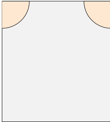
Fig. 5. An additional equilibrium shape that we predict only in dimension two
