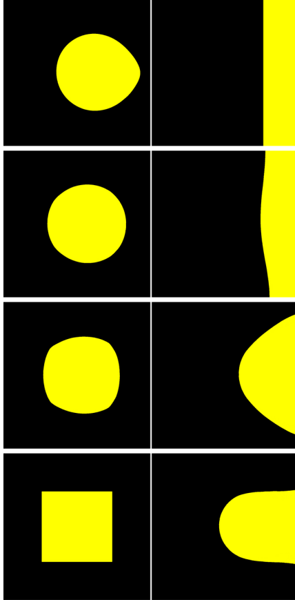
Fig. 2. Numerical simulation of the Muskat problem evolution with a gravity potential. The setup is the same as in Fig. 1 except that the yellow region has a larger mass. The images show snapshots of the evolution at several interesting times. The final configuration is the stationary state, which is qualitatively different from the final configuration in Fig. 1 due to the larger mass
