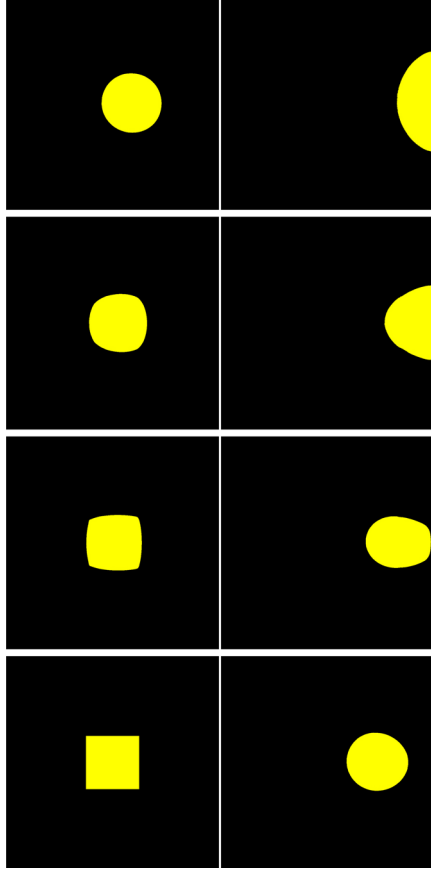
Fig. 1. Numerical simulation of the Muskat problem evolution with a gravity potential. The yellow phase is heavier than the black phase. Under the influence of gravity and surface tension, the yellow phase becomes round and falls. The images show snapshots of the evolution at several interesting times. The final configuration is the stationary state
