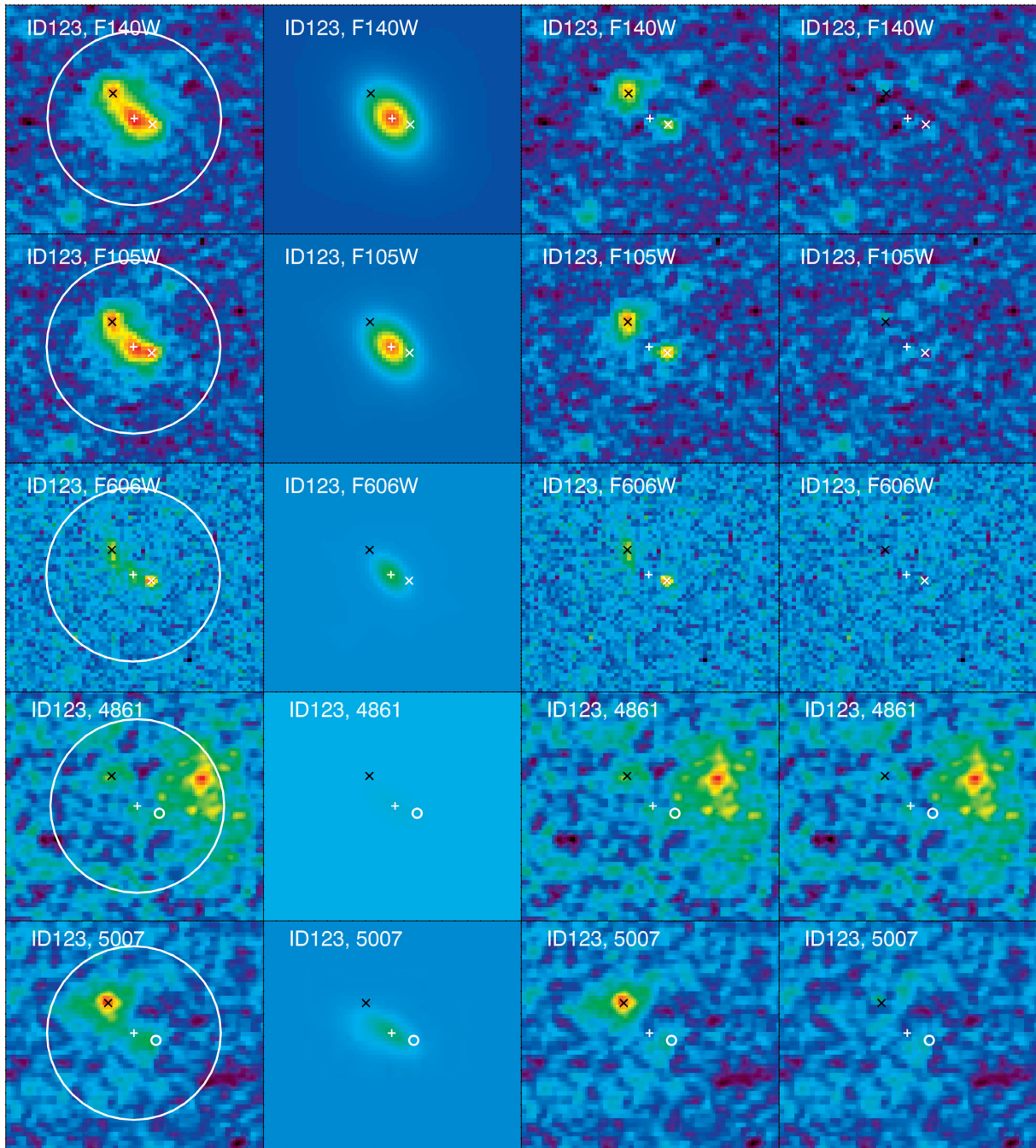
Figure B1. Continuum and emission line maps the galaxy ID123. From top to bottom : F140W , F105W , F606W continuum maps, [O\text{II}] , H\beta , [O\text{III}] , and/or H\alpha emission line maps (the filter or wavelength of the map is indicated in the top left corner of each panel). From left to right : continuum or emission line map, GALFITM model for the diffuse component (single Sérsic profile), residuals obtained subtracting the model (column 2) from the original image (column 1), residuals obtained subtracting GALFITM best-fitting model (including the diffuse Sérsic profile plus additional PSFs at the location of the blobs detected in the residuals shown in column 3) from the original map (column 1). The crosses indicate the centre of the diffuse Sérsic profile. The ‘x’ and small empty circles indicate the centre of the blobs (respectively detected with S/N > 3 or non-detected); white and black are used to indicate blobs with PSF and Sérsic profile. The large white circle indicates the area considered when finding the blobs (and corresponding to five galaxy effective radii). We notice that the [O\text{III}]4959\text{ \AA} is not subtracted in these maps, so it appears as a ‘ghost’ emission in the maps labelled as ‘5007’ (but in the analysis we correct the [O\text{III}]5007\text{ \AA} fluxes for its contribution, Section 2.3). Similarly the [O\text{III}]5007\text{ \AA} is not subtracted from the H\beta maps and therefore it appears as bright blobs in the right-hand side of most of the maps labelled as ‘4861’. In the following, we report the same figure for each galaxy in our sample (the ID is reported in the top left corner of each panel). Each stamp has a size of 3.7\text{ arcsec} \times 3.7\text{ arcsec} ( \sim 30 \times 30\text{ kpc} at z \sim 1-3 ), we adopt the same colour bar in all the panels and an inverse hyperbolic sine scaling. The complete version of this figure is available online.
