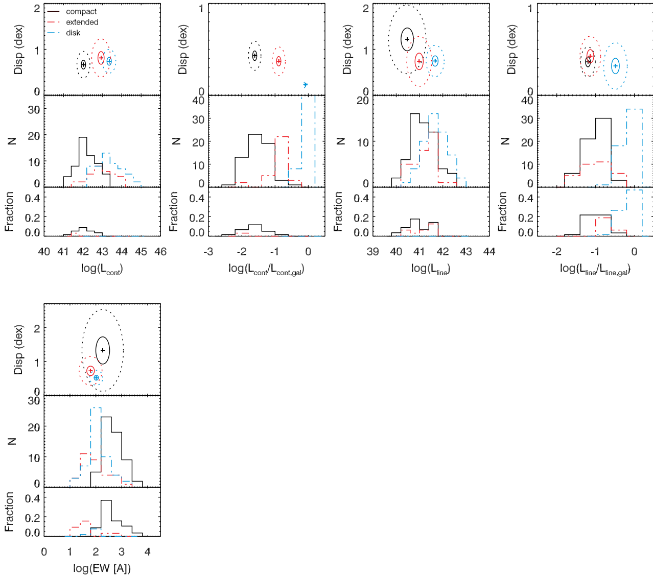
Figure D1. Distribution of the observed properties of blobs and discs. Compact blobs are shown in black, extended ones in red, and the underlying discs in cyan. Top panels (from left to right): We show the distribution of continuum luminosity, continuum luminosity normalized by the total galaxy continuum luminosity, emission line luminosity, and emission line luminosity normalized by the total galaxy line luminosity. Bottom panels (from left to right): We show the distribution of equivalent width. For each observable we show in the middle panel the distribution of the parameters, in the bottom panel the fraction of upper or lower limits in each bin, and in the top panel the mode and dispersion (cross) of each distribution (solid and dotted ellipses indicate the 1\sigma and 3\sigma uncertainty on the mode and dispersion), computed as described in Section 3.6.
