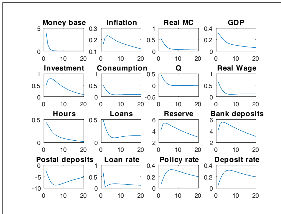
Figure 4: Impulse responses with respect to a positive monetary base shock
