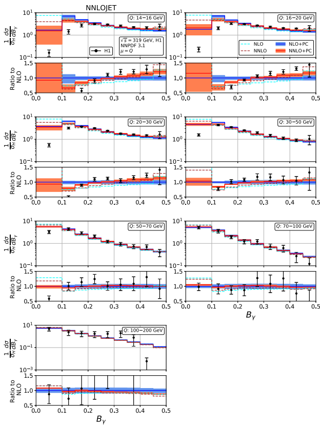
Fig. 12 Event shape distribution for jet broadening with respect to thrust axis: B_\gamma fixed-order predictions at NLO (dashed cyan), NNLO (dashed brown), and corrected for hadronization effects at NLO (blue) and NNLO (red), compared to H1 data [23]. The lower frames display the ratio to the NLO prediction for the central scale \mu^2 = Q^2
