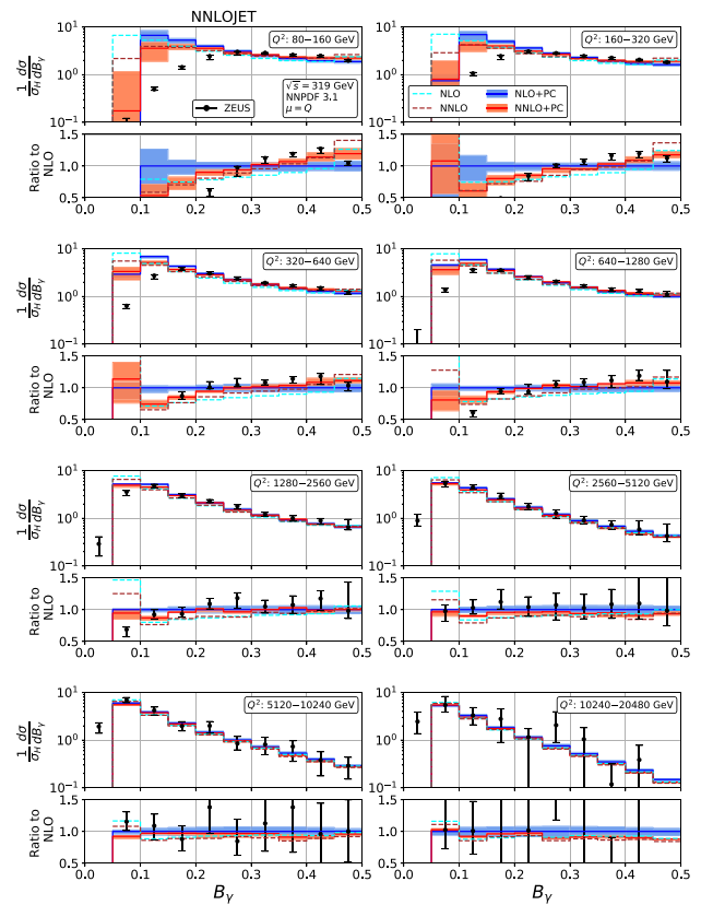
Fig. 13 Event shape distribution for jet broadening with respect to thrust axis: B_\gamma fixed-order predictions at NLO (dashed cyan) and NNLO (dashed brown), and corrected for hadronization effects at NLO (blue) and NNLO (red), compared to ZEUS data [24]. The lower frames display the ratio to the NLO prediction for the central scale \mu^2 = Q^2
