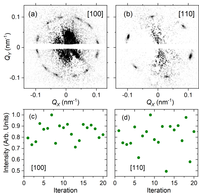
FIG. 6. Sum of images captured for 20 different field cools from 60 K to 20 K at 30 K/min in 54 mT for (a) [100] sample and (b) [110] sample. Intensity of the skyrmion peaks for each measurement normalized to the highest intensity run is shown in (c) for the [100] sample and (d) for the [110] sample.
