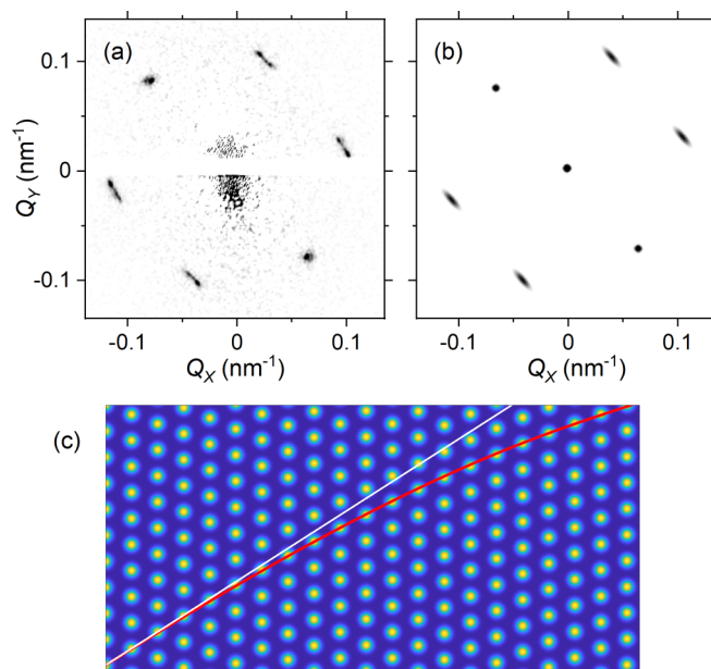
FIG. 7. (a) SAXS pattern of the [100] sample collected at 20 K after field cooling at 10 K/min in 28 mT. (b) Fourier transform of the distorted skyrmion lattice shown below. (c) Schematic of a distorted skyrmion state with shear defects along one direction. The lines are guides to the eye: The red line traces a line of skyrmions in the distorted state, and the white line is a reference straight line where an undistorted lattice would be.
