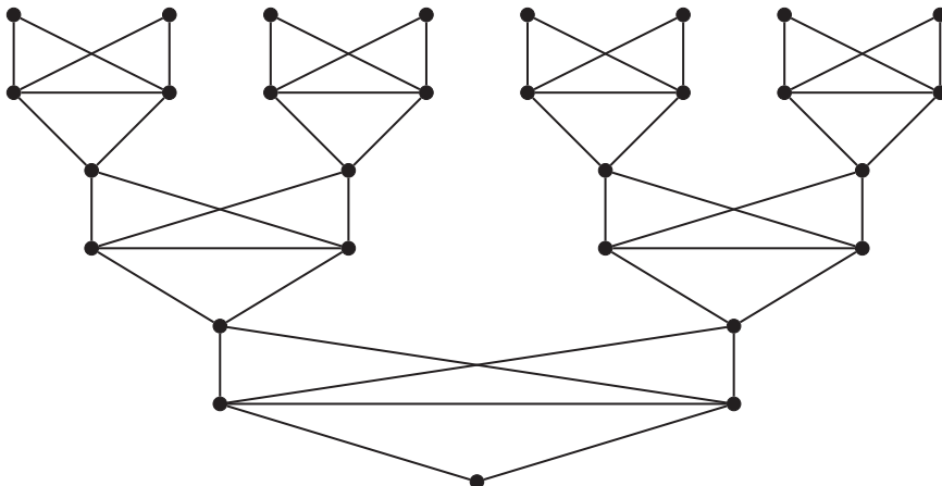
FIGURE 5 The graph H_3^3
