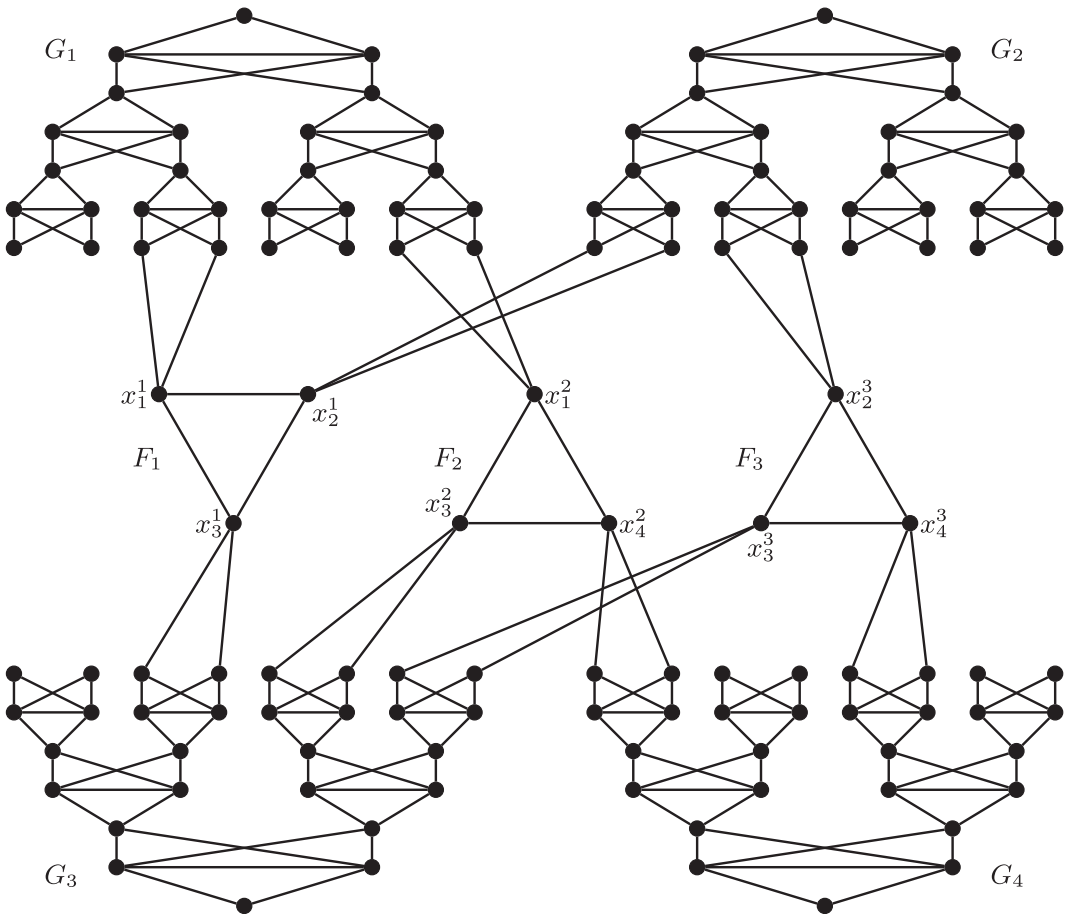
FIGURE 6 The graph G constructed from an instance of 1-IN-3-SAT with C = ((x_1 \vee x_2 \vee x_3), (x_1 \vee x_3 \vee x_4), (x_2 \vee x_3 \vee x_4))
