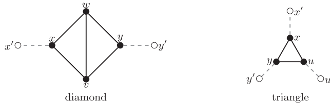
FIGURE 3 The diamond and triangle (solid edges and vertices) together with their neighbourhoods in a cubic graph
