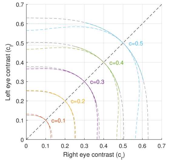
Fig. 2. For each level of standard (diptic) contrast ( c = 0.1 \dots 0.5 ), the color lines show the combination of the left and right eye contrast (dichoptic contrast) that produces the match. The color lines represent the standard and the axis the test conditions in the contrast matching experiment. The lines are plotted according to the contrast matching model from Equation 2 and assuming \beta = 3 . The black-dashed line represents standard contrast. The grey-dashed lines illustrate the range of contrast combinations that result in an unstable percept and rivalry. The color dashed lines illustrate the same relation but according to the late summation model (Equation 3), and the dotted colour lines show the relation in terms of logarithmic contrast (Equation 4).
