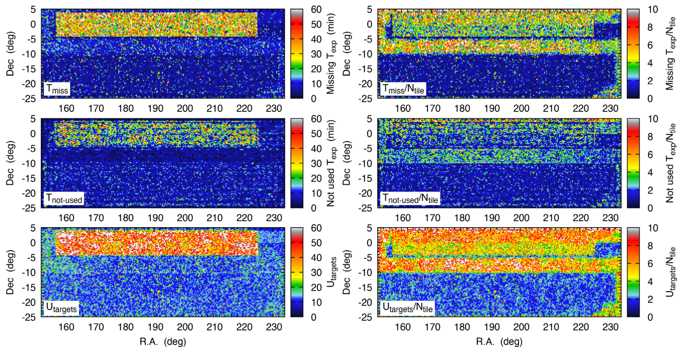
Figure 9. Diagnosis plots of the tiling algorithm. The left-hand column shows the energy function U_{\text{targets}} (lower panel) and its components T_{\text{miss}} (upper panel) and T_{\text{not-used}} (middle panel). In general, T_{\text{miss}} counts the time that is missing to observe the required set of targets and T_{\text{not-used}} counts the time that is wasted because of empty fibres. The U_{\text{targets}} is the combination of these (see Section 3.2.1). The right-hand panels show the same energy function components divided by the number of tiles in a given sky region. This figure shows the energy function components for the tiling presented in the middle panel of Fig. 7.
