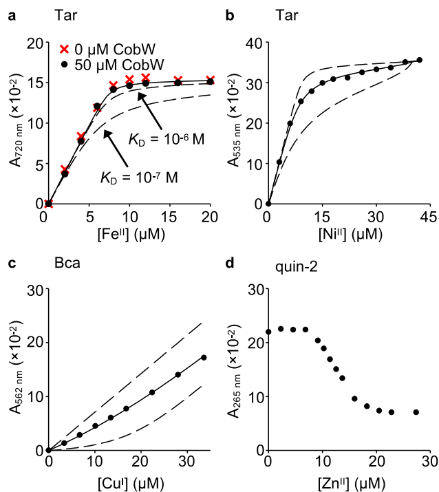
Fig. 3 Binding of \text{Mg}^{\text{II}}\text{GTP-CobW} to \text{Fe}^{\text{II}} , \text{Ni}^{\text{II}} , \text{Cu}^{\text{I}} and \text{Zn}^{\text{II}} . a Absorbance upon \text{Fe}^{\text{II}} titration into a mixture of Tar ( 16\ \mu\text{M} ), \text{Mg}^{\text{II}} ( 2.7\ \text{mM} ) and GTP ( 500\ \mu\text{M} ) in the absence (red crosses) or presence (black circles) of CobW ( 50\ \mu\text{M} ). Dashed lines show simulated responses for specified K_{\text{Fe(II)}} of \text{Mg}^{\text{II}}\text{GTP-CobW} , providing limiting K_{\text{Fe(II)}} \geq 10^{-6}\ \text{M} . Control \text{Fe}^{\text{II}} titration into a solution of Tar ( 16\ \mu\text{M} ) in buffer only (Supplementary Fig. 8a) confirmed that \text{Mg}^{\text{II}} and GTP did not inhibit stoichiometric \text{Fe}^{\text{II}}\text{Tar}_2 formation. b Absorbance change (relative to \text{Ni}^{\text{II}} -free solution) of \text{Ni}^{\text{II}} -titrated Tar ( 20\ \mu\text{M} ) in competition with CobW ( 30\ \mu\text{M} ) in the presence of \text{Mg}^{\text{II}} ( 2.7\ \text{mM} ) and GTP ( 300\ \mu\text{M} ). c Absorbance of \text{Cu}^{\text{I}} -titrated Bca ( 1.0\ \text{mM} ) in competition with CobW ( 20\ \mu\text{M} ) in the presence of \text{Mg}^{\text{II}} ( 2.7\ \text{mM} ) and GTP ( 200\ \mu\text{M} ). In a-c , solid traces show curve fits of experimental data to models where CobW binds one molar equivalent of metal per protein monomer. Supplementary Table 2 contains mean \pm standard deviation (SD) K_{\text{metal}} values from n = 3 independent experiments (full details in Supplementary Figs. 8–12 and Supplementary Table 1). In b, c , dashed lines show simulated responses for K_{\text{metal}} tenfold tighter or weaker than the fitted value. d Absorbance (relative to probe-free solution) upon titration of \text{Zn}^{\text{II}} into a mixture of quin-2 ( 10\ \mu\text{M} ), \text{Mg}^{\text{II}} ( 2.7\ \text{mM} ), GTP ( 100\ \mu\text{M} ) and CobW ( 10\ \mu\text{M} ).
