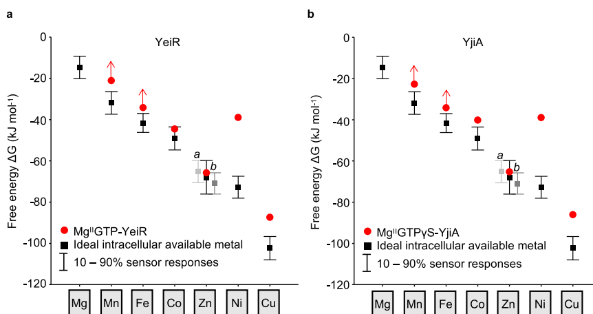
Fig. 6 \text{Mg}^{\text{II}}\text{GTP-YeiR} and \text{Mg}^{\text{II}}\text{GTP}\gamma\text{S-YjiA} preferentially acquire \text{Zn}^{\text{II}} . a Free-energy change ( \Delta G ) for metal binding to \text{Mg}^{\text{II}}\text{GTP-YeiR} (red circles) plotted against the intracellular available free energies for metal binding (as described in Fig. 5; black squares and bars). b As a for \text{Mg}^{\text{II}}\text{GTP}\gamma\text{S-YjiA} (red circles). Arrows indicate where only a limiting \Delta G was determined (thus \Delta G > plotted value).
