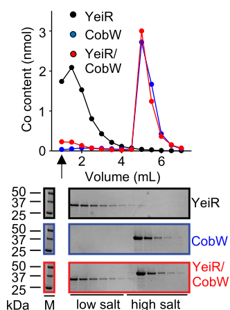
Fig. 7 Mg II GTP-CobW outcompetes Mg II GTP-YeiR for Co II . Elution profile of YeiR (10 \mu M), CobW (10 \mu M) or both proteins following incubation with GTP (100 \mu M), Mg II (2.7 mM) and Co II (8 \mu M) resolved by differential elution from an anion exchange column. Fractions were analysed for Co II by ICP-MS and protein by SDS-PAGE (YeiR alone black, CobW alone blue, both proteins red; n = 1 ). Arrow denotes flow through fractions. Full gel images and SDS-PAGE analysis of flow through fractions shown in Supplementary Fig. 26.
