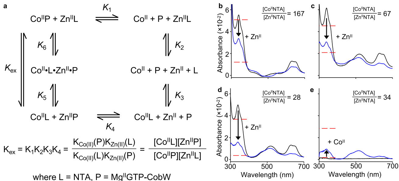
Fig. 4 Mg II GTP-CobW binds Zn II with sub-picomolar affinity. a Representation of the equilibrium for exchange of Co II and Zn II between ligand (L = NTA) and protein (P = Mg II GTP-CobW). b–e Absorbance (relative to metal-free solution) of solutions of CobW (17.9–20.4 μM), Mg II (2.7 mM), GTP (200 μM) and NTA (0.4–4.0 mM) upon (b–d) first addition of Co II (black trace) then Zn II (blue trace) or (e) the reverse, at equilibrium ( n = 1 for each panel). The absorbance peak at 339 nm corresponds to Co II -bound protein. An excess of ligand NTA was used to buffer both metals in each experiment: varying the ratios of ligand-bound metal ions ([Co II NTA]/[Zn II NTA] = 28–167) shifted the ratios of Co II - and Zn II -bound protein as predicted by the equilibrium exchange constant in a. Consistent K Zn(II) values for Mg II GTP-CobW were generated at all tested conditions (Supplementary Table 4). Dashed red lines show expected A 339 nm peak intensities for K Zn(II) of Mg II GTP-CobW tenfold tighter or weaker than calculated values.
