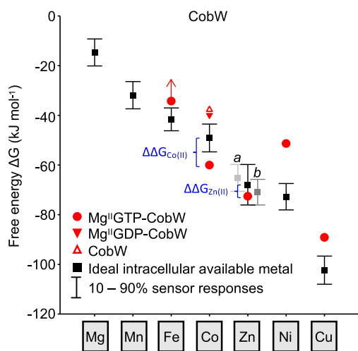
Fig. 5 Mg II GTP-CobW is predicted to acquire Co II or Zn II in a bacterial cell. Free-energy change ( \Delta G ) for metal binding to Mg II GTP-CobW (red circles) plotted against the intracellular available free energies for metal binding in a reference bacterial cytosol (values correspond to Salmonella ) under idealised conditions (i.e. where each metal sensor undergoes half of its transcriptional response; black squares). Intracellular available \Delta G_{\text{Zn(II)}} is the mean of the values determined from the two Zn II sensors ZntR (a) and Zur (b). Bars show the change in intracellular available \Delta G as cognate sensors shifts from 10–90% of their responses. Free energy differences ( \Delta\Delta G ) which favour acquisition of metals by Mg II GTP-CobW in vivo are indicated in blue. \Delta G values for Co II complexes of CobW alone (open red triangle) and Mg II GDP-CobW (closed red triangle) are also shown. For Fe II binding to Mg II GTP-CobW, arrow indicates limiting \Delta G > -34.2 \text{ kJ mol}^{-1} .
