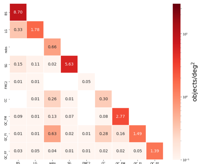
Figure 13. Heat map showing the target density of GAMA galaxies ( z > 0.002 ) that are missed in the BGS. The diagonal shows the number of objects per deg 2 removed by each of the individual spatial and photometric cuts applied in the BGS, while the off-diagonal entries show the densities of objects removed by both cuts labelled on the x and y axes.
