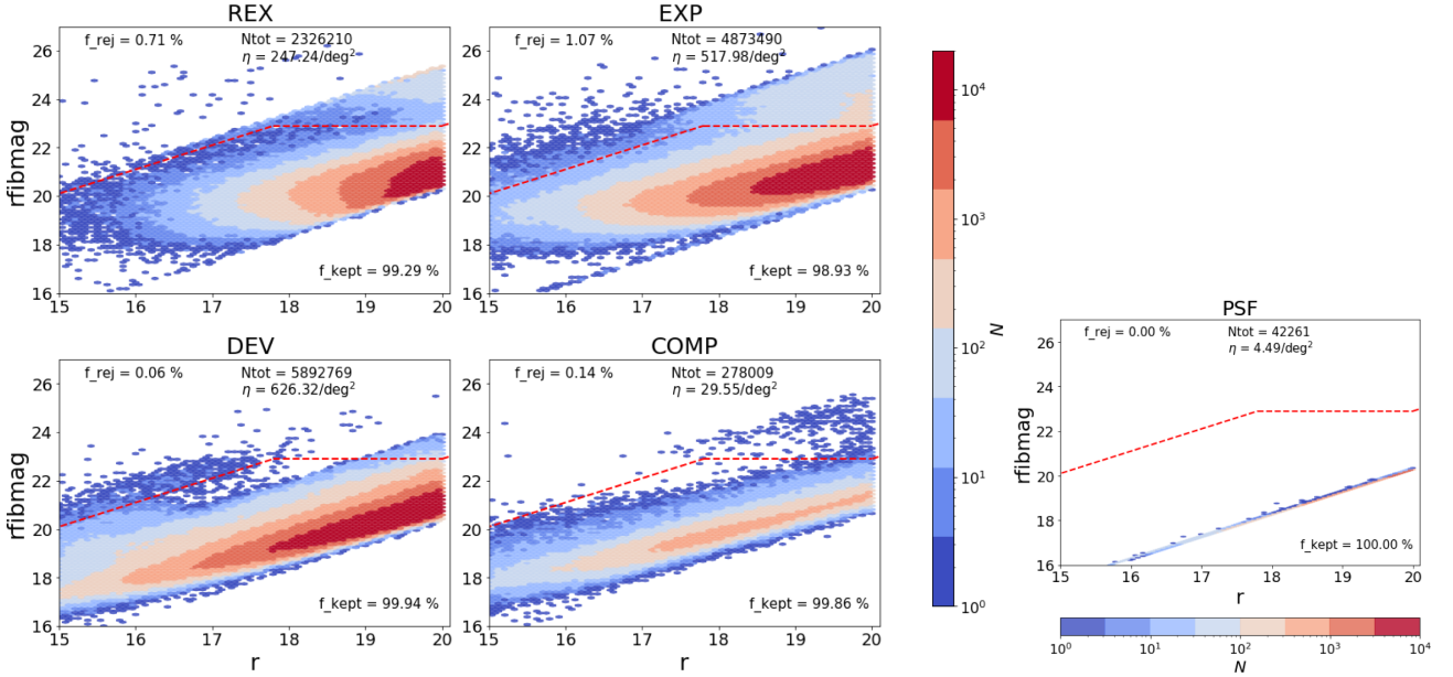
Figure 6. BGS galaxies in the r -band total magnitude ( x -axis) versus r -band fibre magnitude ( y -axis) plane in the LS DR8. The results are divided into the five different TRACTOR best-fitting light profile models, as labelled at the top of each panel. The colour bar shows the number counts of objects in a hexagonal cell covering the range from 1 to 20000 for four of the light profile models with the exception of PSF-type galaxies, in which case the scale covers 1 to 10000. The red-dashed line shows the fibre magnitude cut (FMC): we reject every object that is above this threshold. The numbers shown in top left-hand and bottom right-hand corners give the fraction of galaxies rejected and kept, respectively, while the number in the top right-hand corner shows the total number of galaxies ( N_{\text{tot}} ) and the corresponding target density ( \eta ).
