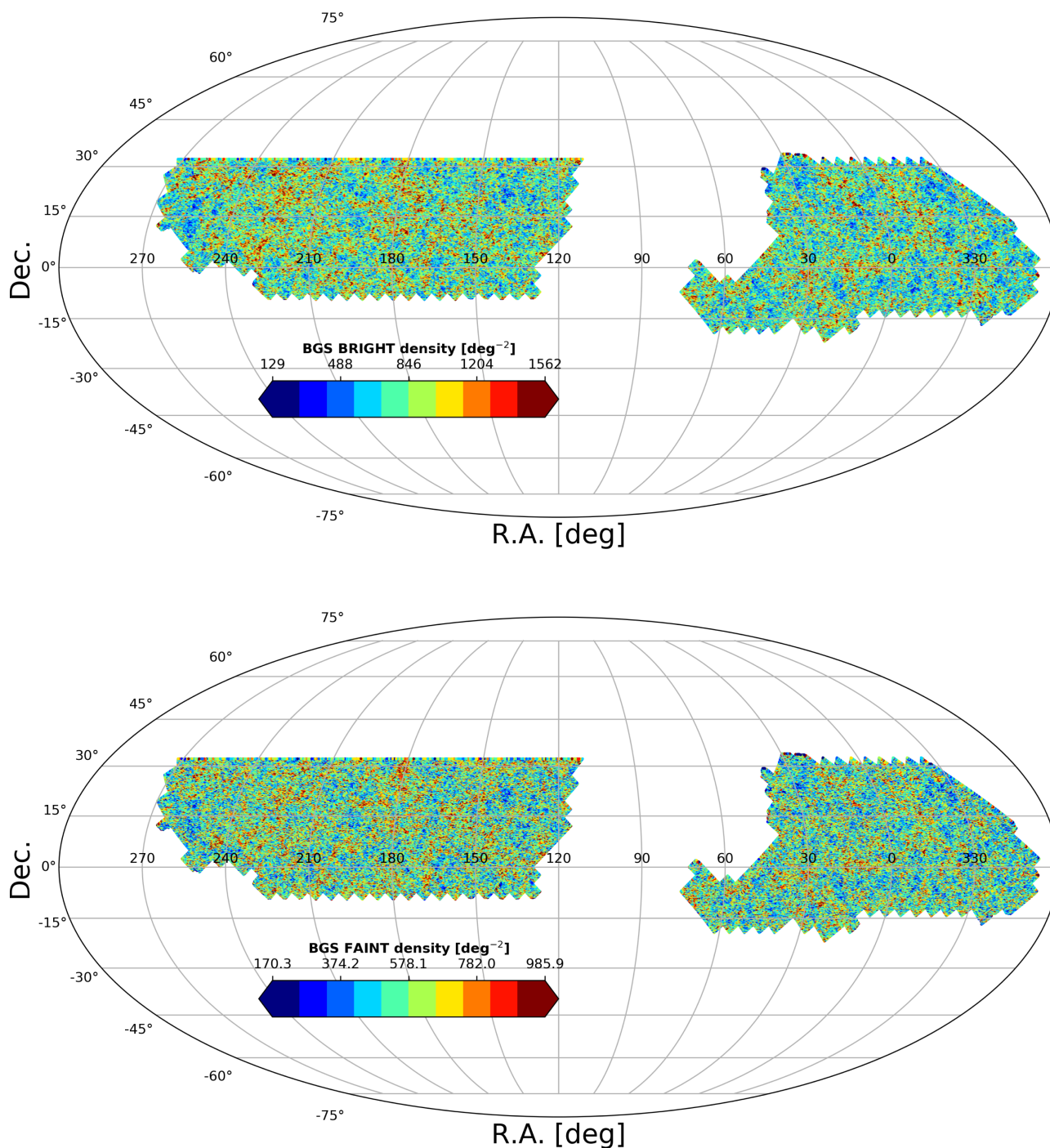
Figure 8. The distribution on the sky of the BGS BRIGHT (upper map) and BGS FAINT (lower map) target density in objects \text{deg}^{-2} , computed on a HEALPIX grid with a resolution of N_{\text{side}} = 256 . The mean densities are 846 and 579 objects \text{deg}^{-2} for the bright and faint BGS, respectively.
