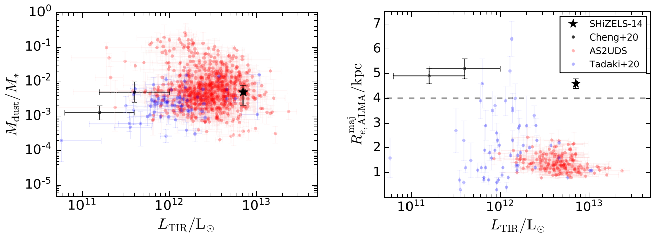
Figure 9. Left-hand panel: dust mass-to-stellar mass ratio versus total infrared luminosity, for the AS2UDS submillimetre bright galaxies (red circles; Dudzeviciute et al. 2020), the subset of stellar mass-selected galaxies from Tadaki et al. (2020) that are in UDS and have size measurements, and the three TIR-brightest SHiZELS galaxies from Cheng et al. (2020) (black). SHiZELS-14 (black star) is well within the range of both parameters derived for the submillimetre galaxy population. Dust mass and stellar mass are derived using MAGPHYS for SHiZELS-14 and the AS2UDS and Tadaki et al. (2020) samples. Right-hand panel: effective radius (along the semimajor axis) versus total infrared luminosity for the subsample of these galaxies targeted at higher spatial resolution with ALMA, presented by Gullberg et al. (2019), 2 with the small statistical correction derived by Smail et al. (2021) applied to the source sizes. The grey line at R_{e, \text{ALMA}} = 4 kpc marks the effective radius of the faint extended component that is measured in the stacking analysis of Gullberg et al. (2019). For both the Gullberg et al. (2019) sample and SHiZELS-14, radii were calculated using 2D Sérsic fits (with fixed n = 1 ) in the image plane. For the remaining SHiZELS galaxies, radii were derived using a curve-of-growth analysis (Cheng et al. 2020). For the Tadaki et al. (2020) sample, radii were derived using Gaussian model fits in the uv plane. SHiZELS-14 has a much larger effective radius (as measured in the rest-frame FIR) than the majority of the AS2UDS galaxies, though several less FIR-luminous galaxies in the Tadaki et al. (2020) sample are similarly extended. The extended dust emission suggests that SHiZELS-14 is caught in the mid-stages of a merger.
