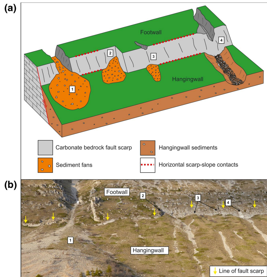
Figure 3. (a) Schematic diagram of slope processes that can lead to nontectonic exhumation and burial of active limestone fault scarps. Labels 1–4 indicate areas of hangingwall erosion or deposition that are inappropriate sample locations. Ideal sites are located tens of meters away from areas affected by depositional and erosional slope processes, where the scarp-slope contacts are horizontal, after Bubeck et al. (2015). (b) The Campo Felice fault with features from (a) indicated. Photo taken from (42.2308°N, 13.4343°E), view northeast. The horizontal scale is approximately 320 m across image at the height of scarp.
