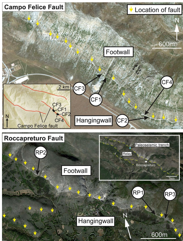
Figure 4. Location of sites used in this study, inset in the top panel shows the length of the Campo Felice fault. Campo Felice sites CF1, CF2, and CF3 were sampled during this study, and site CF4 was sampled and processed by Benedetti et al. (2013). On the Roccapreturo fault (lower panel), sites RP1 and RP2 were sampled during this study, and site RP3 was sampled and processed by Schlagenhauf (2009). The inset panel shows the relay where two strands of the RP fault overlap. Imagery from Google Earth, 2018.
