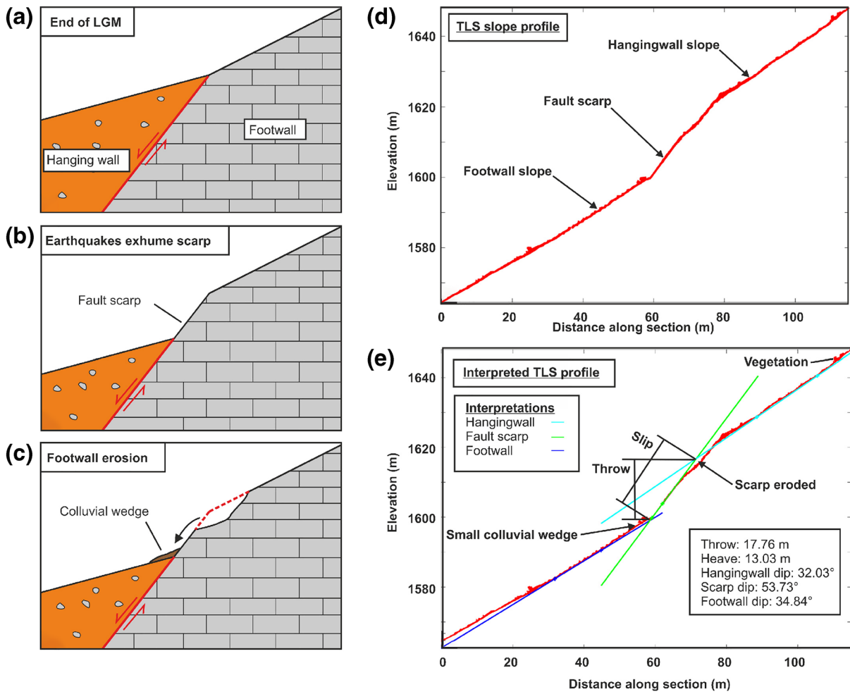
Figure 2. (a) Schematic model of fault scarp development when exhumation rate is slower than erosion rate, as was the case during the LGM in the Central Italian Apennines. (b and c) show a schematic model of scarp evolution since the end of the LGM, when exhumation rate outpaces erosion rate. Panel (d) shows a typical fault-perpendicular profile, from the Campo Felice fault, through a point cloud generated from TLS data and (e) shows one profile interpretation. Samples are not collected from the eroded section of the fault scarp due to the uncertainty in the timing of erosion; only the planar lower section is sampled. LGM, Last Glacial Maximum; TLS, Terrestrial Laser Scanning.
