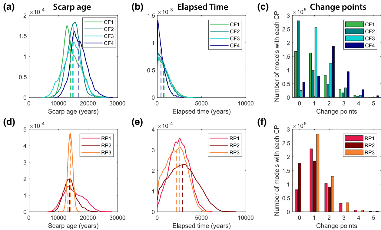
Figure 10. Posterior probability distribution functions from all models for scarp age (a and d) and elapsed time parameters (b and e), for each fault with each site plotted as different colored lines. The vertical dashed lines correspond to the median of each distribution. The number of models with each number of change points for each site is shown in (c and f).
