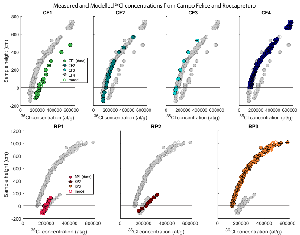
Figure 5. 36 Cl concentration versus sample height in the plane of slip at each locality. Each filled point represents a different sample, and each suite of colored points represents data from one site as indicated. Site data are plotted on top of data from the same fault (in gray) on each plot for comparison. Open circles show the modeled 36 Cl from the MAP (maximum a posteriori estimation). The color scheme for each site is kept uniform in the figures that follow. Data from Campo Felice Site CF4 are from Benedetti et al. (2013), and data from Roccapreturo Site RP3 are from Schlagenhauf (2009). Analytical 1 \sigma uncertainties are plotted as black lines. These are raw 36 Cl values, and some variation in 36 Cl between sites and noise in sample data is related to different production rates resulting from variable Ca, which is corrected in the forward model.
