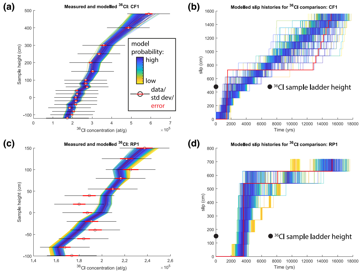
Figure 8. Figures (a and c) show the fit to data of models used to calculate average fault slip rates, for sites CF1 and RP1. The circles and error bars represent the ^{36}\text{Cl} measurements and the standard deviation of the data (used in the likelihood calculation); each colored line represents a model, with dark to light colors representing highest to lowest probability models, regulated by the scarp age probability and the number of change points. We present 400 models for each site ranging from the highest (dark blue) to lowest (yellow) probability at equal intervals (100) through the distribution. Figures (b and d) represent the corresponding model slip histories. The full distributions from the inversion for each site can be found in the supporting information.
