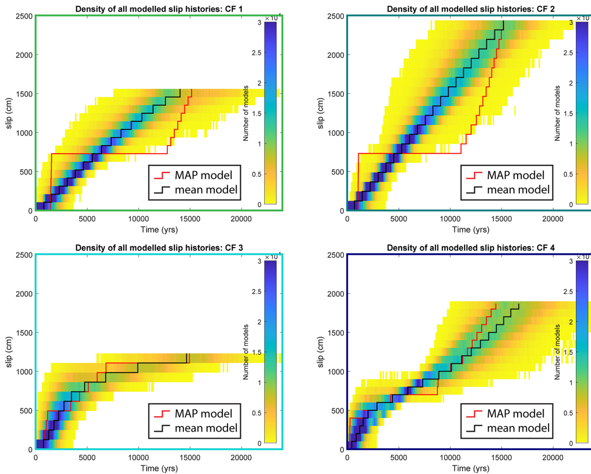
Figure 6. MCMC Modelling results from the Campo Felice fault ^{36}\text{Cl} data. Each subfigure includes 500k iterations as a 2D histogram showing the distribution of accepted slip histories in time-slip space. The distribution reflects the density of overlapping models, but does not capture the pattern of any individual slip history. The red line is the maximum a posteriori probability (MAP) estimation model, which is the maximum likelihood multiplied by the prior probability based on scarp age. The black line represents the mean model—which is the mean time for each slip step. MCMC, Markov chain Monte Carlo.
