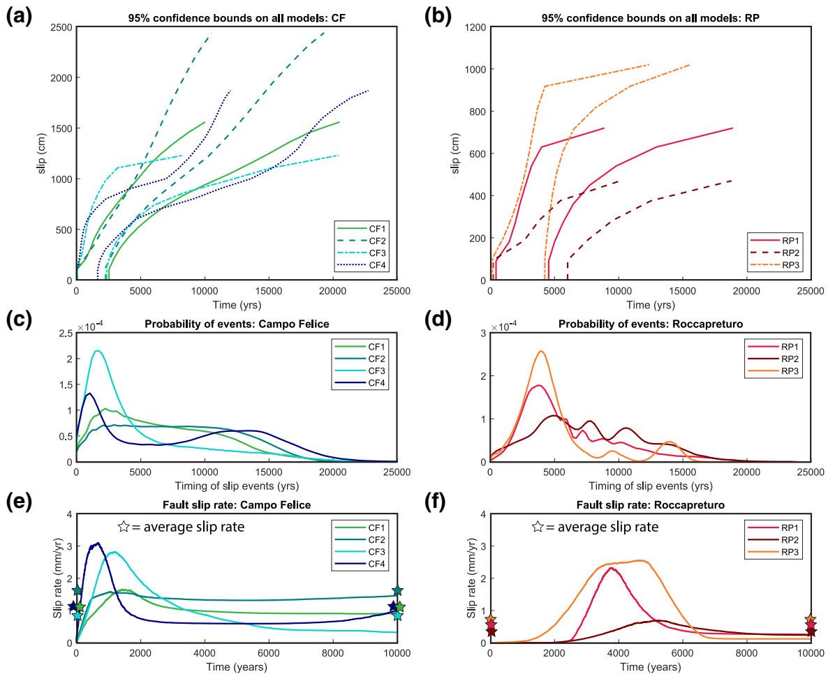
Figure 7. Summary of MCMC results from the Campo Felice and Roccapreturo faults. Panels (a and b) show the 95% confidence bounds on models from each site. Panels (c and d) show the probability distribution of slip events over time (for the full model results). Panels (e and f) show the average slip rate for the top 10% most probable models over time, in 1 year bins, and stars indicate the average slip rate calculated based on the median scarp age and scarp height. Note the different time scale for panels (e and f). MCMC, Markov chain Monte Carlo.
