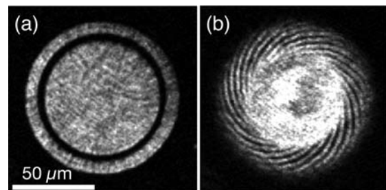
Fig. 13. (a) A ring trap with a diameter of 100 μm is created using a repulsive DMD-patterned potential combined with an attractive horizontal sheet beam. By using the dynamic control of the DMD, a stirring barrier is introduced into the ring and then accelerated through 90°, before being removed from the ring. The resulting persistent current is imaged through interference with the central BEC in a short time of flight, determining a net circulation quanta of N = 21 .
