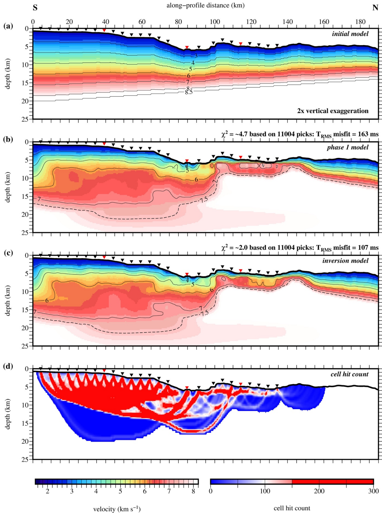
Supplementary Figure S2. Inversion modelling starting with the sloping bottom initial model (cf. Fig. 4). a) Initial model. b) Phase 1 interim model. c) Final model. See text and Table 1 for approach and parameters adopted. \chi^2 fit, the root-mean-square misfit ( T_{\text{RMS}} ) and the number of travel time picks are labelled for each stage. Velocity contours are plotted at 1.0 \text{ km s}^{-1} intervals, together with the 7.5 \text{ km s}^{-1} contour used as a proxy for base of crust. d) Cell hit count. In all parts, OBS locations are marked by inverted black triangles, with OBSs 001, 113 and 125 highlighted in red.
