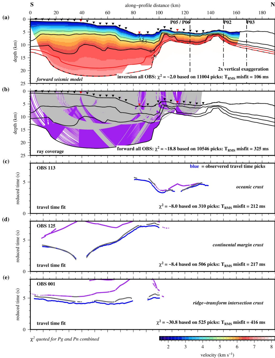
Figure 9. Forward ray-tracing to constrain the Moho and SITF. a) Forward seismic model derived from the P-wave inversion model and using the 5.5 \text{ km s}^{-1} contour to mark the boundary between the upper and lower crust. P-wave inversion model ' 7.0 and 7.5 \text{ km s}^{-1} contours are shown for reference as solid and dashed red lines respectively. OBS locations are shown (black inverted triangles), with OBSs 001, 113 and 124 highlighted in red. CAYSEIS Profiles P05/P06, P02 and P03 (left to right) are marked by the dot-dashed lines. b) Ray diagram for OBSs 001, 113 and 125, showing travel times point-to-point traced as both Pg and Pn phases (grey ray paths), and a predictive trace of where PmP arrivals (purple ray paths) should be observed. See text for discussion. c-e) Time-distance graphs for OBSs 113 (oceanic crust), 125 (continental crust) and 001 (ridge-transform intersection crust) showing the ray traced arrivals (Pg and Pn – grey; PmP – purple) compared with observed arrivals (blue) with dot size set to pick error. The predicted PmP arrivals are shown on the corresponding data sections in Fig. 3. \chi^2 fit, the root-mean-square misfit ( T_{\text{RMS}} ) and the number of travel time picks are labelled for each stage.
