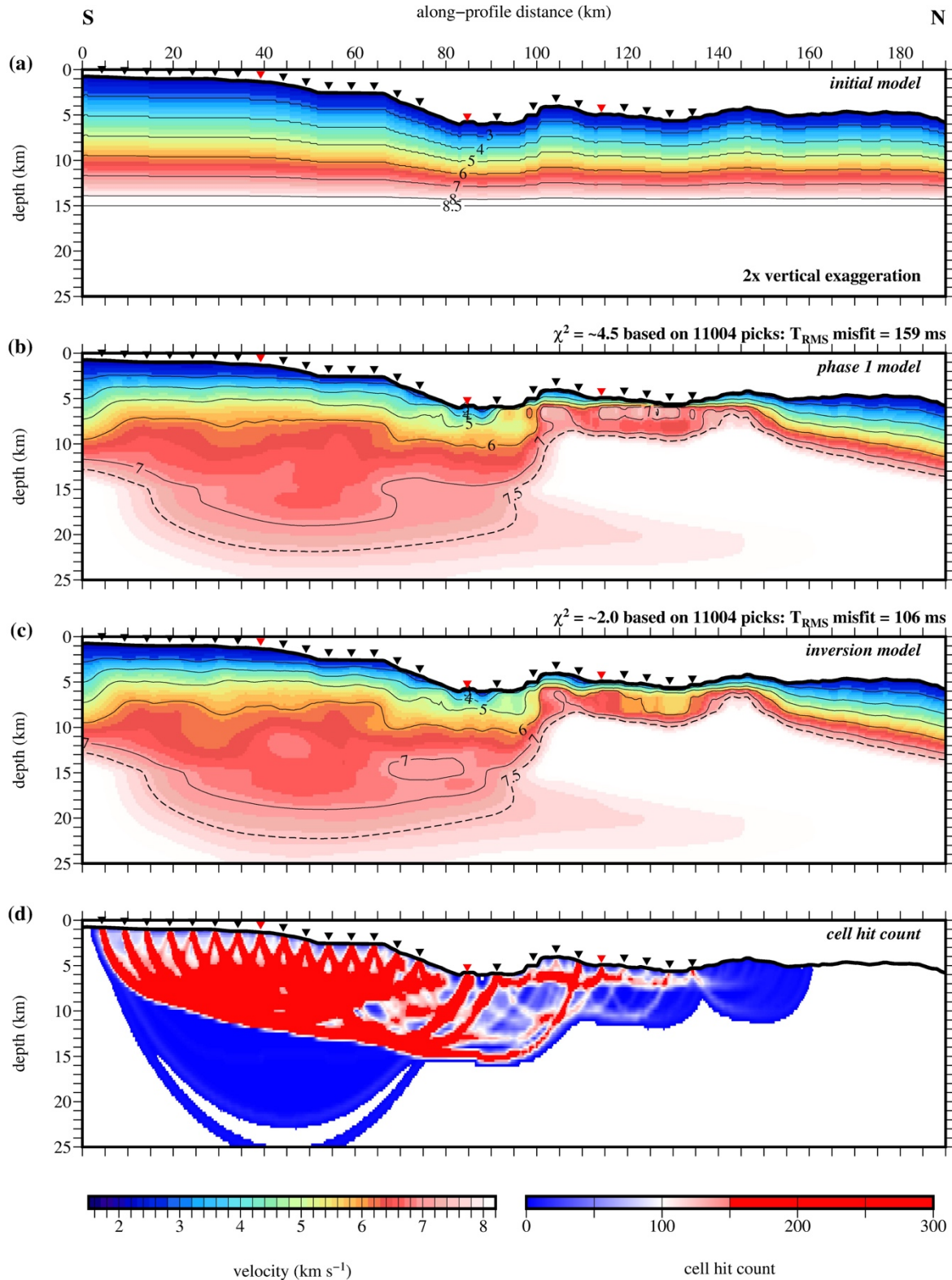
Figure 5. Inversion modelling. a) P -wave initial model. b) Phase 1 interim model. c) Best-fit P -wave inversion model. See text and Table 1 for approach and parameters adopted. \chi^2 fit, the root-mean-square misfit ( T_{\text{RMS}} ) and the number of travel time picks are labelled for each stage. Velocity contours are plotted at 1.0 \text{ km s}^{-1} intervals, together with the 7.5 \text{ km s}^{-1} contour used as a proxy for base of crust. d) Cell hit count indicatively showing ray coverage used to mask the P -wave inversion model in other figures. In all parts, OBS locations are marked by inverted black triangles, with OBSs 001, 113 and 125 highlighted in red.
