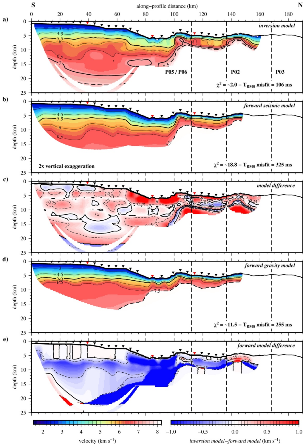
Figure 14. Comparison between P-wave velocity-depth models resulting from inversion and forward approaches to modelling. a) P-wave inversion model . b) Forward seismic model . c) Calculated velocity difference between the two models, contoured at 0.25 \text{ km s}^{-1} intervals. d) Forward gravity model . e) Calculated velocity difference between the forward seismic model and the forward gravity model , contoured at 0.25 \text{ km s}^{-1} intervals. See text for discussion. The 5.5 \text{ km s}^{-1} velocity contour marks the transition from upper-to-lower crust and the 7.5 \text{ km s}^{-1} contour (dashed) denotes the Moho. OBS locations are shown (black inverted triangles), with OBSs 001, 113 and 125 highlighted in red. CAYSEIS Profiles P05/P06, P02 and P03 (left to right) are marked by the dot-dashed lines. \chi^2 fit and root-mean-square misfit ( T_{\text{RMS}} ) are labelled.
