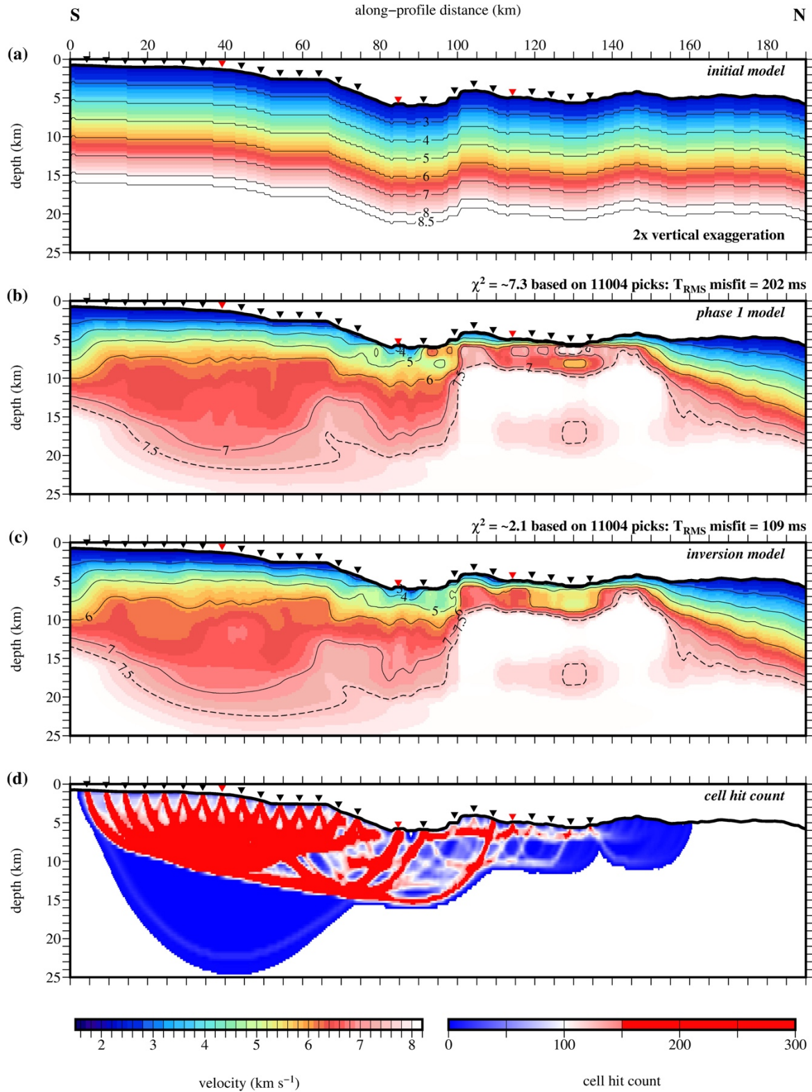
Supplementary Figure S1. Inversion modelling starting with the seabed following initial model (cf. Fig. 4). a) Initial model. b) Phase 1 interim model. c) Final model. See text and Table 1 for approach and parameters adopted. \chi^2 fit, the root-mean-square misfit ( T_{\text{RMS}} ) and the number of travel time picks are labelled for each stage. Velocity contours are plotted at 1.0 \text{ km s}^{-1} intervals, together with the 7.5 \text{ km s}^{-1} contour used as a proxy for base of crust. d) Cell hit count. In all parts, OBS locations are marked by inverted black triangles, with OBSs 001, 113 and 125 highlighted in red.
