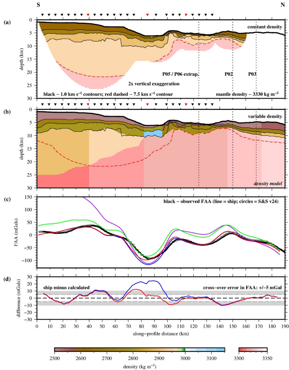
Figure 8. Gravity modelling test of the P -wave inversion model. a) Density-depth model with solid black lines marking the 4.0, 5.0 and 6.0 km s -1 velocity contours, and the red dashed line the 7.5 km s -1 velocity contour used as block boundaries initially. Constant densities were applied to blocks within the same layer. Dotted vertical lines mark Profiles P05/P06, P02 and P03 (left to right) intersections. OBS locations are marked by inverted black triangles, with OBSs 001, 113 and 125 highlighted in red. b) Density model with variable densities within each layer, together with a gradation in density within the mantle, required to achieve the best-fit to the observed free-air anomaly (FAA). At the SITF (82 to 96 km along-profile distance) higher densities are required in the lower crust/upper mantle. See text for discussion and interpretation. c) Observed (ship – black line; Sandwell and Smith, 2009 v24 – open circles) and calculated (coloured lines) FAAs, showing that higher density crust at the SITF is required to achieve a fit. Coloured lines represent anomalies calculated on the basis of: constant density blocks within layers with blocks defined solely by velocity contours (purple); constant density blocks within layers with blocks adjusted to achieve a longer wavelength fit (green); variable density blocks within layers consistent with their continental or oceanic location (blue); and variable density blocks including a higher density region beneath the SITF (red) required to achieve the best-fit. d) Misfit of the variable block density models plotted against FAA error bound.
