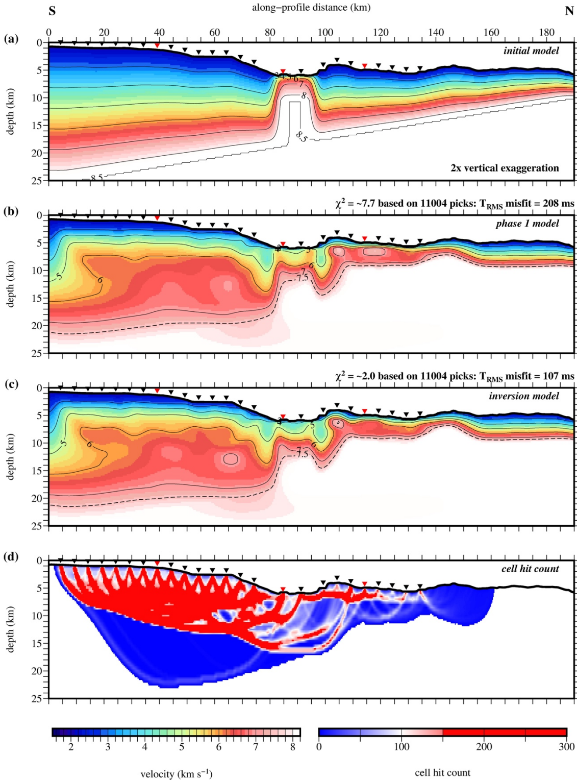
Figure 10. Inversion modelling of SIFT crustal structure using a seeded initial model based on the density model . a) P -wave initial model. b) Phase 1 interim model. c) Best-fit seeded inversion model. Approach and inversion parameters were kept as summarized in Table 1. \chi^2 fit, the root-mean-square misfit (T RMS ) and the number of travel time picks are labelled for each stage. Velocity contours are plotted at 1.0 km s -1 intervals, together with the 7.5 km s -1 contour used as a proxy for base of crust. d) Cell hit count indicatively showing ray coverage used as the mask in Fig. 11. In all parts, OBS locations are marked by inverted black triangles, with OBSs 001, 113 and 125 highlighted in red.
