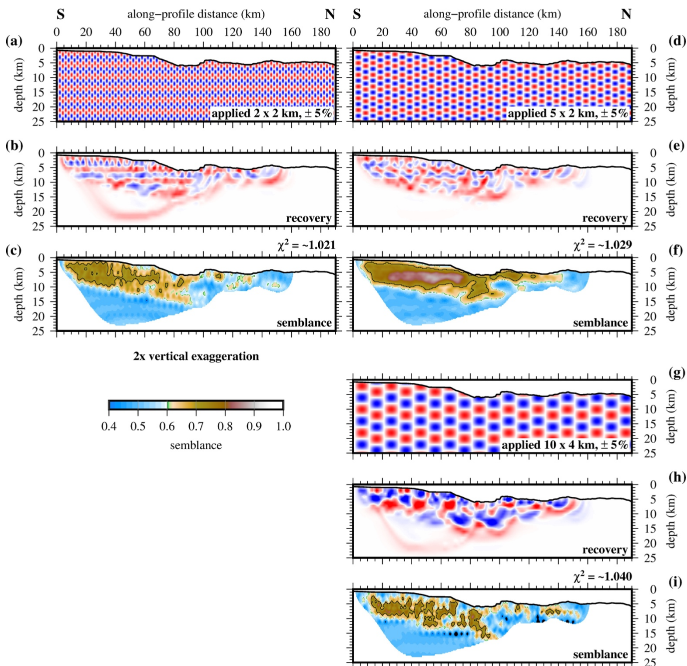
Figure 11. Checkerboard resolution testing of the seeded inversion model . a) Checkerboard applied to the seeded inversion model with a 2 x 2 km pattern size and 5% velocity anomaly. b) Recovered checkerboard. c) Semblance masked by ray coverage. A semblance of 0.7 is used as the good resolution threshold. \chi^2 fit is annotated. A good resolution is achieved for the top ~5-7 km of the continental crust. d-f) Checkerboard testing with a 5 x 2 km and 5% velocity anomaly checkerboard. A good resolution is achieved to ~10 km depth in the continental crust and a better resolution is achieved beneath the SITF, and to ~3-5 km beneath the MCSC. g-i) Checkerboard testing with a 10 x 4 km and 5% velocity anomaly checkerboard.
