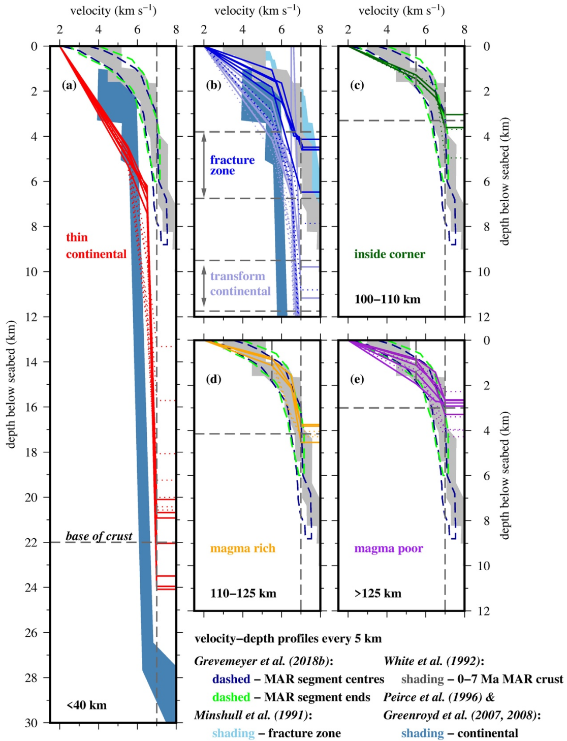
Figure 13. P -wave forward (solid lines) and inversion (dotted lines) model velocity–depth profiles. One-dimensional profiles, extracted at 5 km intervals, are colour-coded by setting along-profile: a) continental crust; b) transform continental and fracture zone crust; c) ridge-transform intersection; d) magma rich; and e) magma poor oceanic crustal formation. Average crustal thicknesses are marked (horizontal grey dashed lines). Profiles are compared to the Atlantic crustal velocity–depth envelopes of White et al. (1992) (grey shaded) and Grevmeyer et al. (2018b) (blue dashed = MAR segment centre crust; green dashed = MAR segment end crust), continental crustal (blue shaded) compilations of Peirce et al. (1996) and Greenroyd et al. (2007, 2008), and the fracture zone compilation (light blue shaded) of Minshull et al. (1991).
