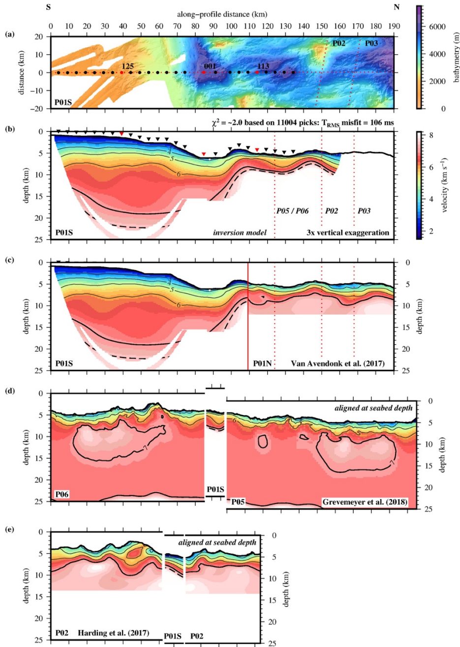
Figure 7. Comparison between CAYSEIS P-wave inversion models. a) Swath bathymetry surrounding Profile P01S. OBS locations (black dots/inverted triangles) shown in all parts, with OBSs 001, 113 and 125 (red dots/inverted triangles) highlighted. Profiles P01, P05 & P06 (extrapolated) and P02 & P03 (intersecting along the northern end of Profile P01 as a whole) are marked by red dotted lines. b) P-wave inversion model for Profile P01S. c) Comparison between the inversion model of this study for the southern section of Profile P01 (P01S) and that of Van Avendonk et al. (2017) for the northern section (P01N), showing a very good correlation, despite different approaches to inversion being adopted, over the ~40 km overlap. d) Comparison between P-wave velocity-depth models for Profiles P06 and P05 (Grevemeyer et al., 2018) and Profile P01S at the MCSC. e) Comparison between the P-wave velocity-depth models for Profile P02 (Harding et al. 2017) and P01S at their intersection. In parts b-e) velocity contours are plotted at 1.0 km s -1 intervals (thin black lines), with the 7.0 km s -1 contour shown by a thick black line. The 7.5 km s -1 contour (black dashed line) is used as a proxy to define the Moho.
