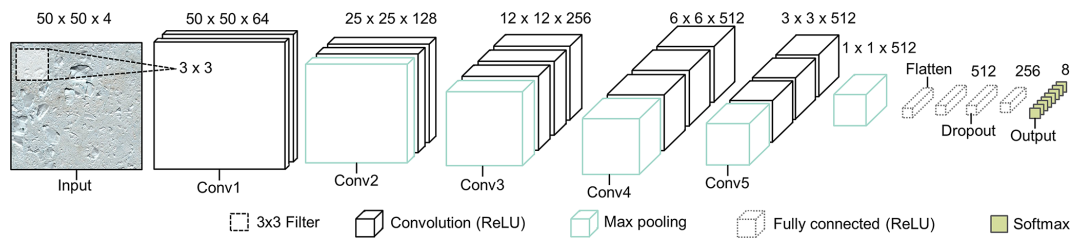
Figure 4. Architecture of phase one CNN, adapted from the original VGG16 model architecture (Simonyan and Zisserman, 2015). Diagram shows an example with a 50 \times 50 px RGBNIR input image tile. There are five stacks of 2D convolutional layers (labelled “Conv#”) which extract features from input tiles using a 3 \times 3 filter. The convolutional stacks are followed by a fully connected neural network and Softmax activation for phase one class prediction. The Sentinel-2 image in this figure is courtesy of the European Union Copernicus programme.
