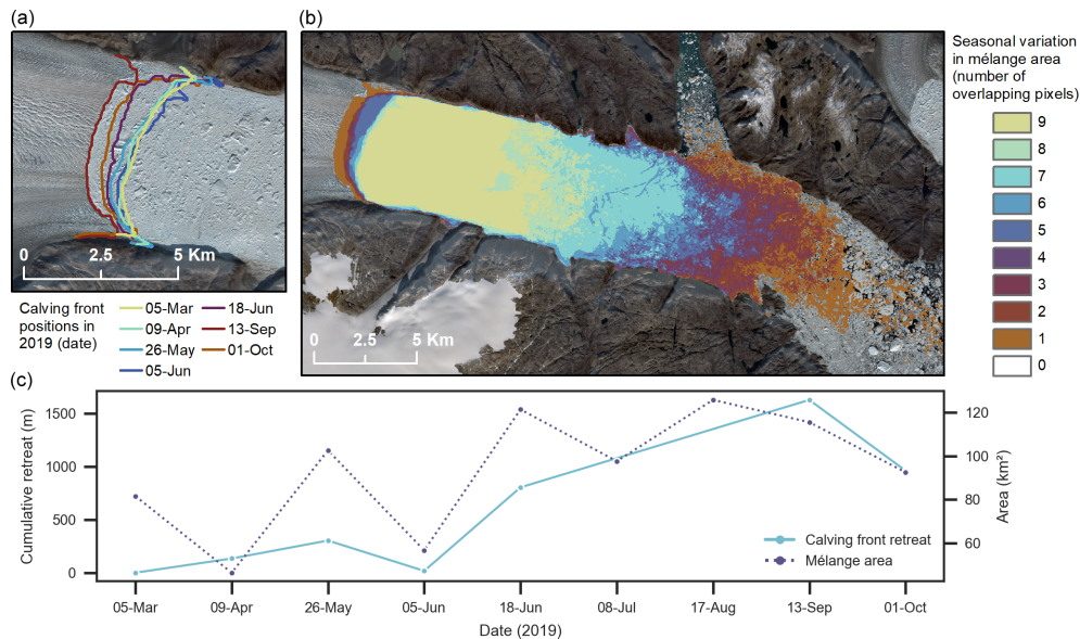
Figure 10. (a) Time series of Helheim calving front positions produced from CSC outputs of the 2019 test data. (b) Frequency of CSC-predicted mélange pixels from the Helheim test dataset showing the seasonal variation in mélange extent. (c) Cumulative retreat of the calving front relative to 5 March 2019 and mélange area for each test image. All background Sentinel-2 imagery in this figure has been made available courtesy of the European Union Copernicus programme.
