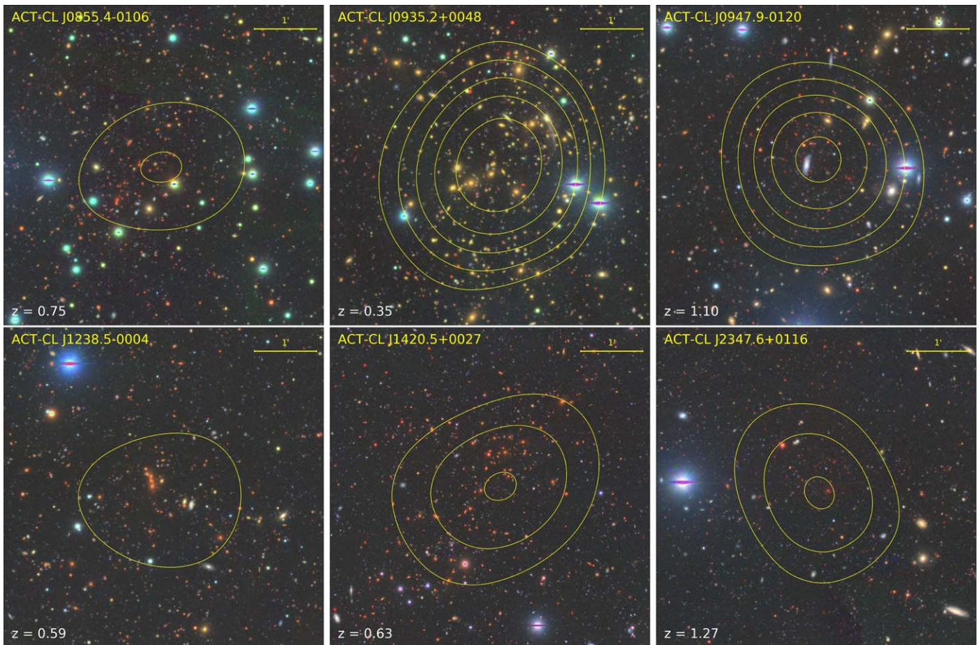
Figure 11. Example gri images of ACT DR5 clusters at various redshifts, confirmed using HSC imaging and the CAMIRA optical cluster finder. Each image is 5' on a side, with north at the top and east at the left. The ACT S/N contours have the same scaling as in Figure 10.
