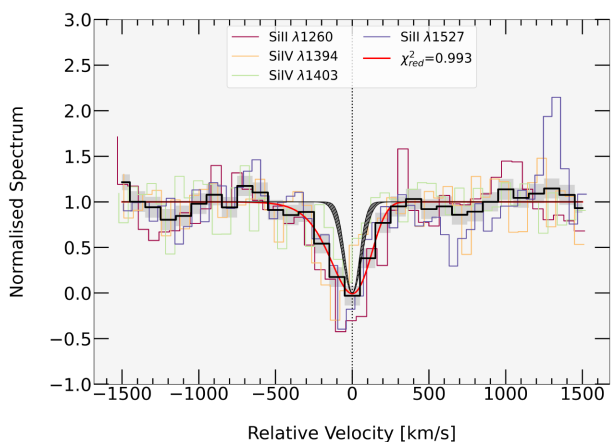
Figure 9. Diagram showing the normalized profile of the strongest FUV absorption lines as a function of the line-of-sight velocity (rest frame). The black solid line shows the mean profile of the absorptions, while the grey shaded area is indicative of the 1\sigma uncertainty. The grey hatched Gaussian represents the range of resolution in velocity of MUSE obtained from equation (8) in Bacon et al. (2017). The red solid line shows the best fit of the stacked spectrum performed with a skewed Gaussian model.
